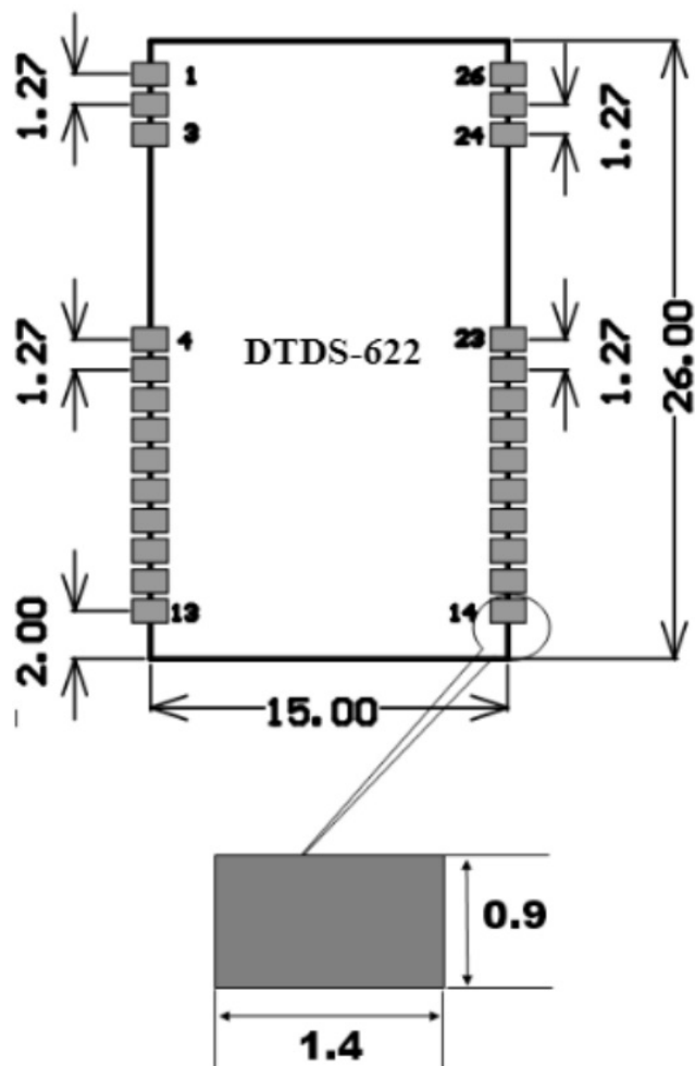
Figure 3- Physical Dimensions of the DTDS-622C Module (all units are in mm)
