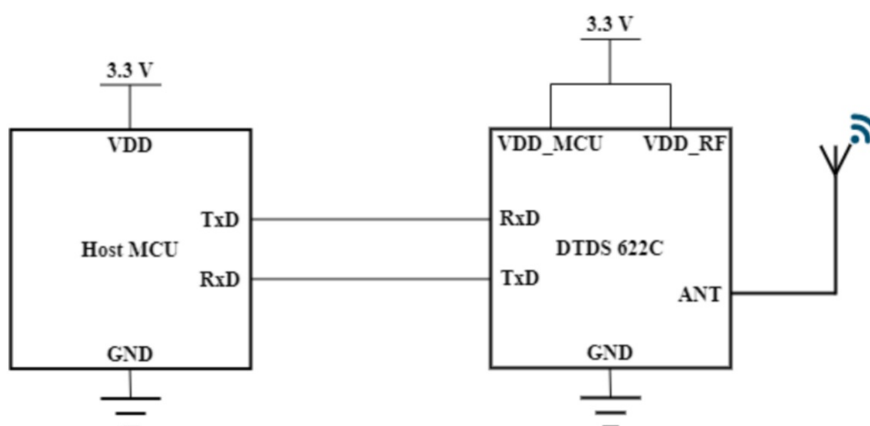
Figure 2- Connection Diagram for User Application
