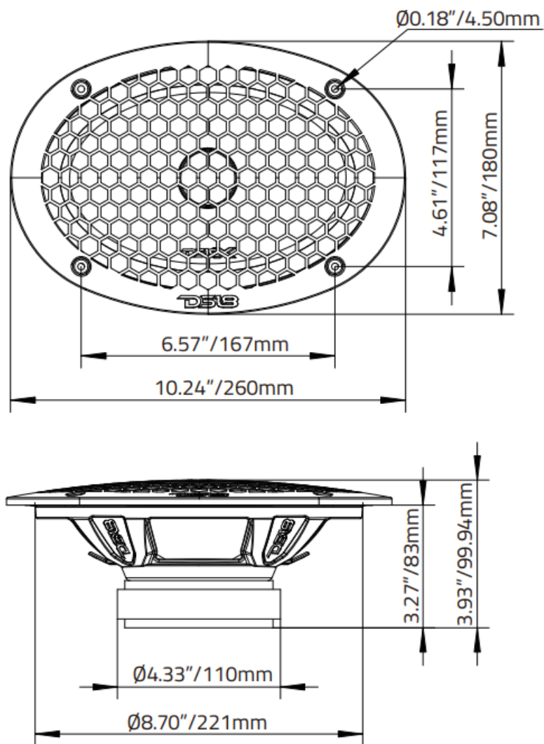
PRO-X698BM 6×9" MID-RANGE LOUDSPEAKER WITH BULLET
