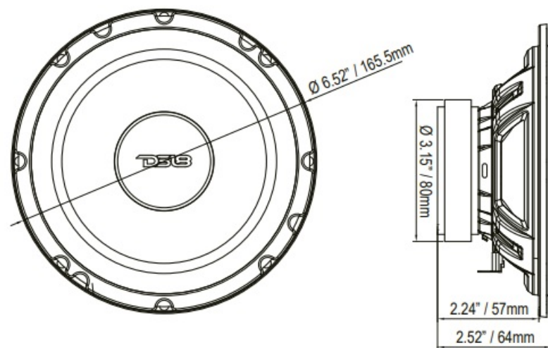
MEASUREMENTS / MEDIDAS: WOOFER
