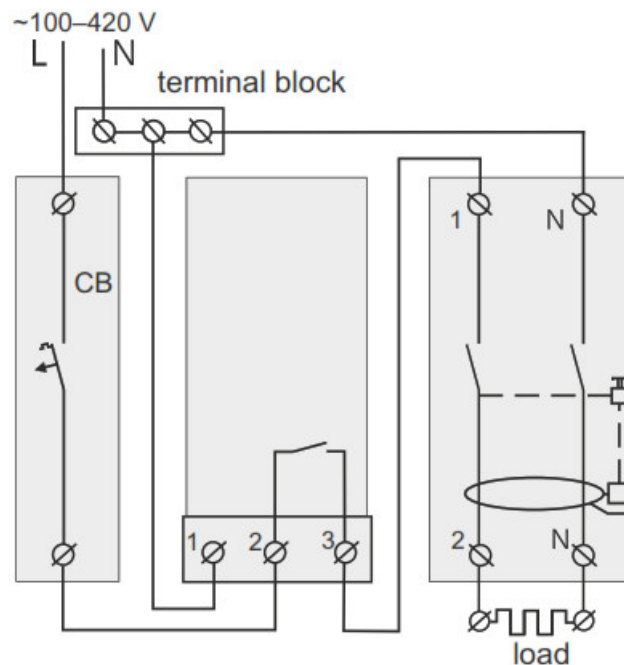
Scheme 2. Connection of the circuit breaker and SSD (safety shutdown device)
