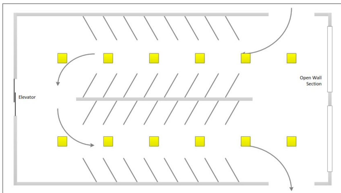
Fig. 1 One level of a small, multi-level parking garage having 12 luminaires positioned over two drive lanes. Each luminaire is equipped with an FMS. This level has an open wall section (a daylighting opportunity) on the far right and a pedestrian access point (elevator) on the far left.
