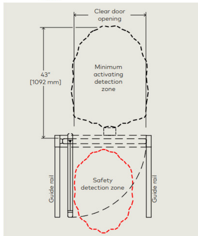
Fig. 5.1.1 One way traffic, overhead mounted safety sensor
