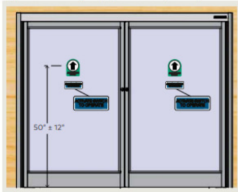
Fig. 7.5.3 Knowing act, approach side, one way
