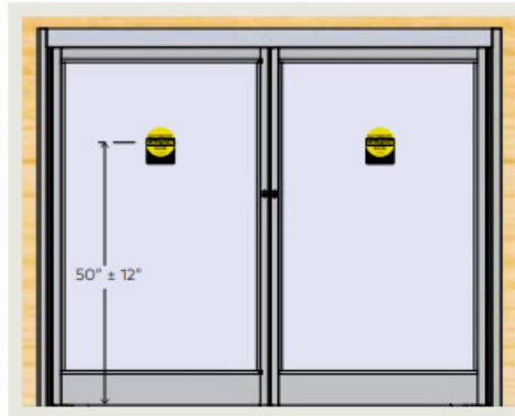
Fig. 7.5.6 Knowing act, swing side, one way
