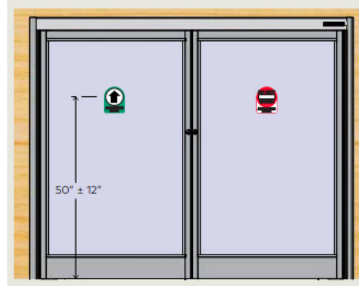
Fig. 7.7.6 LH double egress, exterior side
