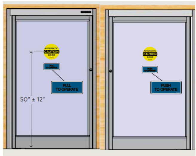
Fig. 7.4.2 Push/Pull Push To Operate
