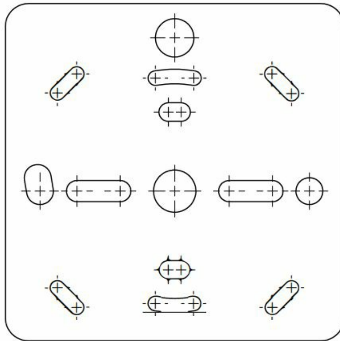
Drill and Tap Template Apexx Series Lock
