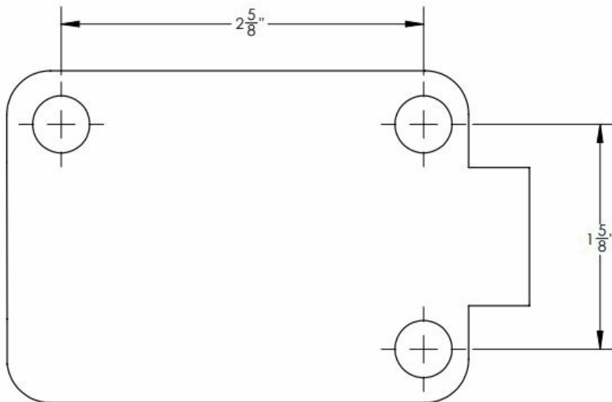
Drill and Tap Template Apexx Series Lock
