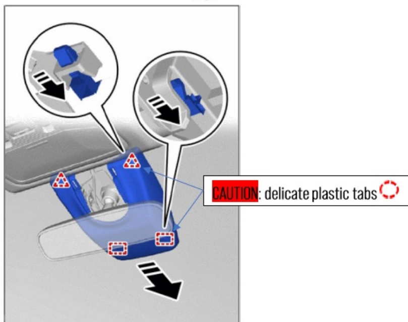
Figure 3: Outer plastic shroud removal
