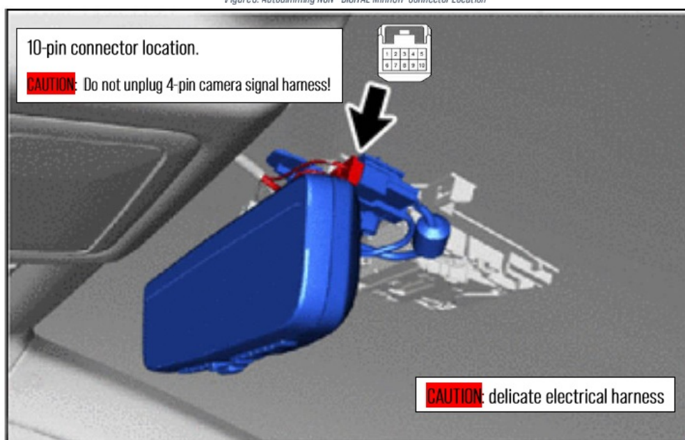
Figure 4: Digital Mirror Connector Location
