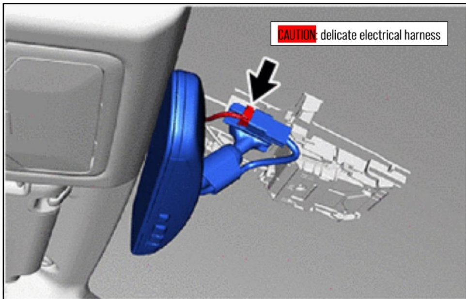
Figure 3: Autodimming NON-"DIGITAL MIRROR" Connector Location
