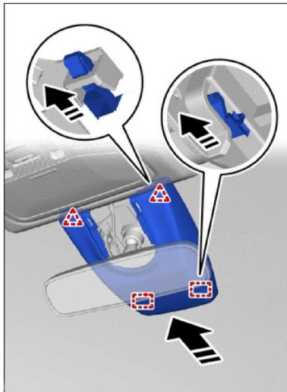
Figure 6: Outer plastic shroud reinstallation
