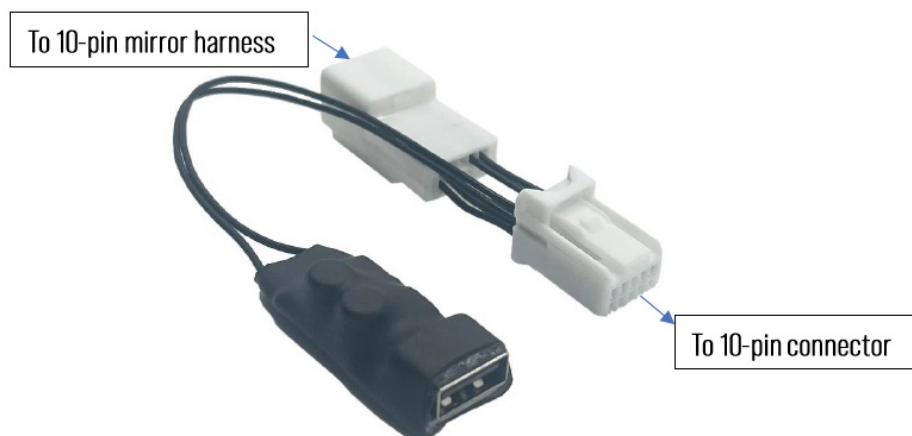
Figure 5: 10-pin Type B adapter
