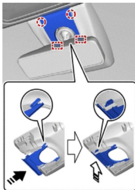
Figure 7: Inner plastic shroud reinstallation
