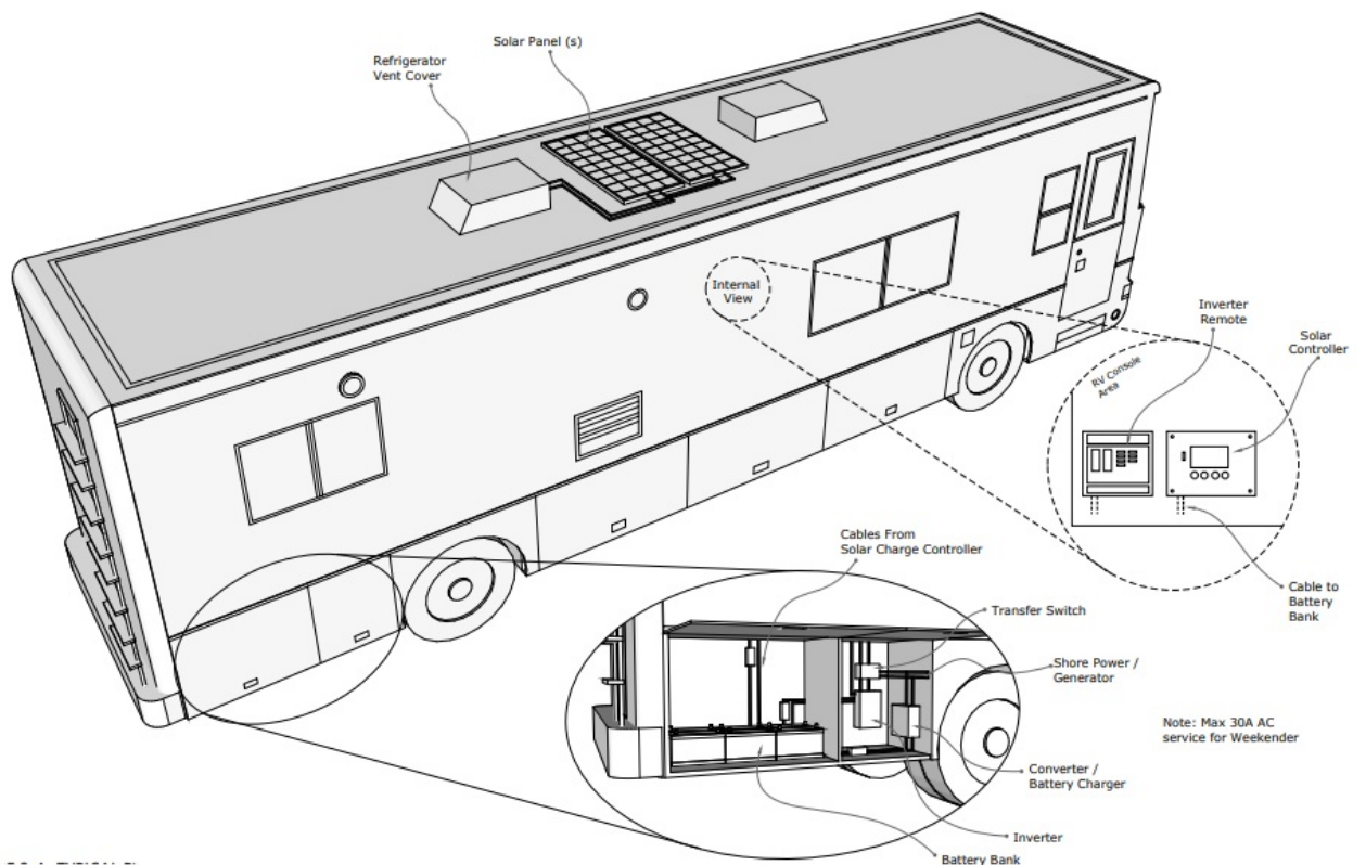
FIGURE 2-B: ECLIPSE 190 WIRING DIAGRAM
