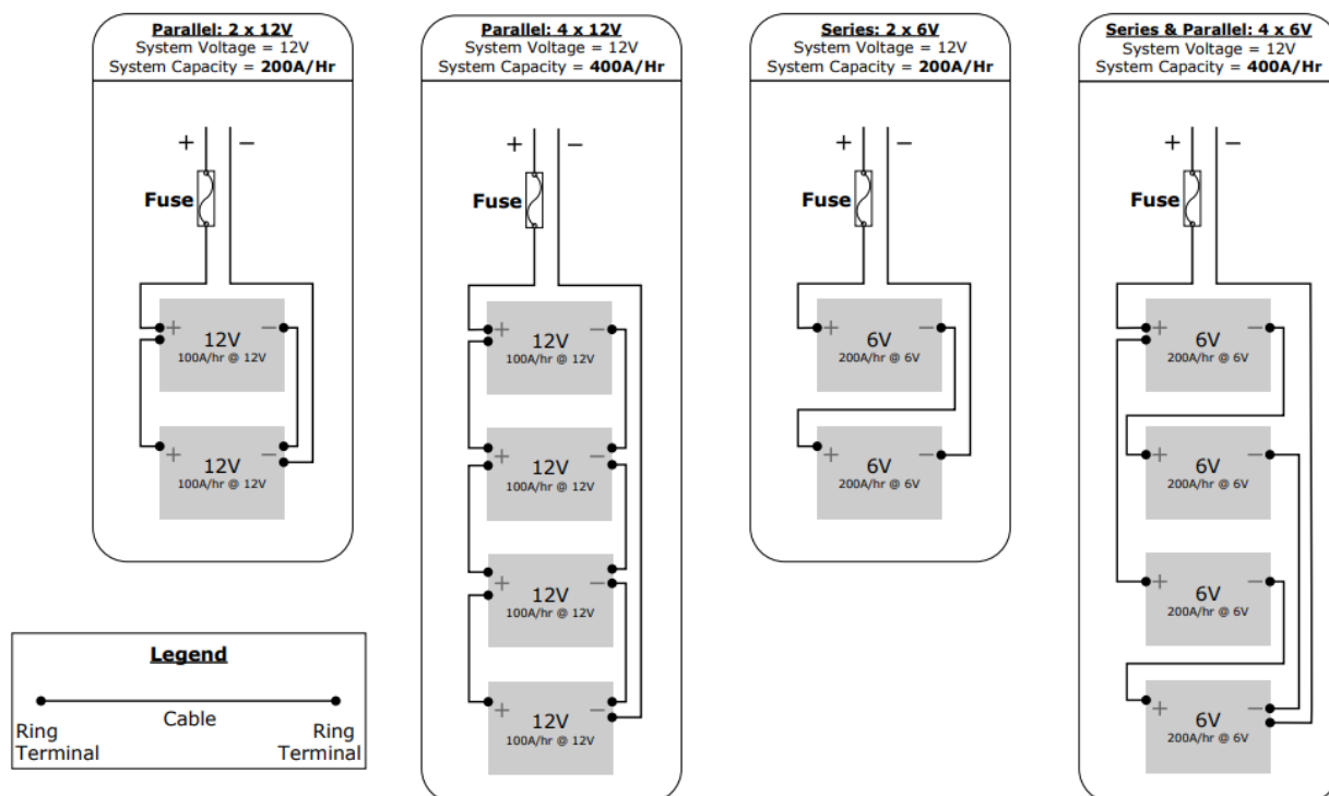
FIGURE 4-J: TYPICAL BATTERY BANK CONFIGURATIONS
