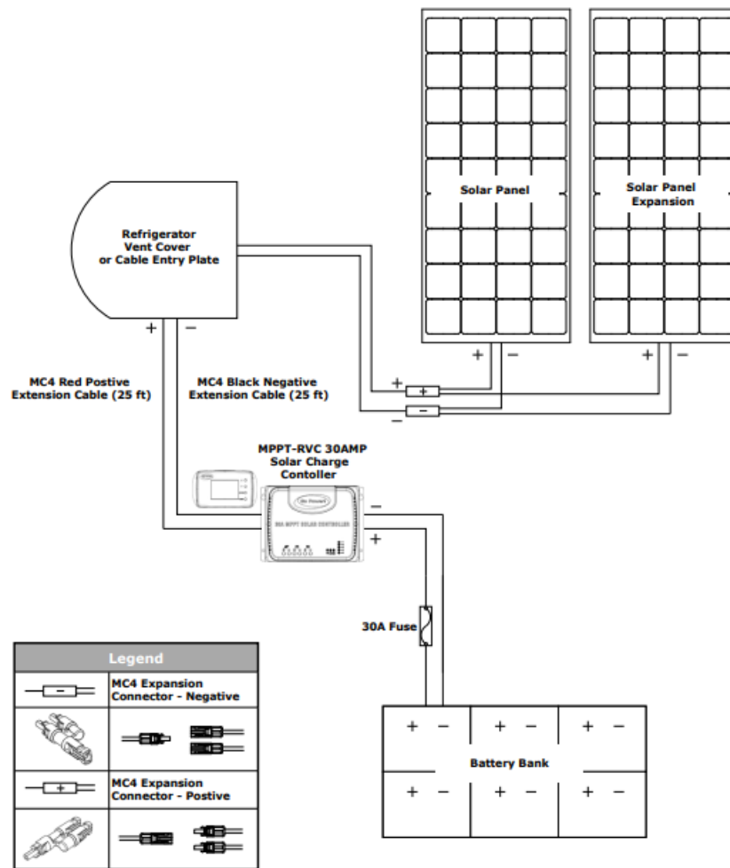
FIGURE 2-B: ECLIPSE 190 + EXPANSION WIRING DIAGRAM
