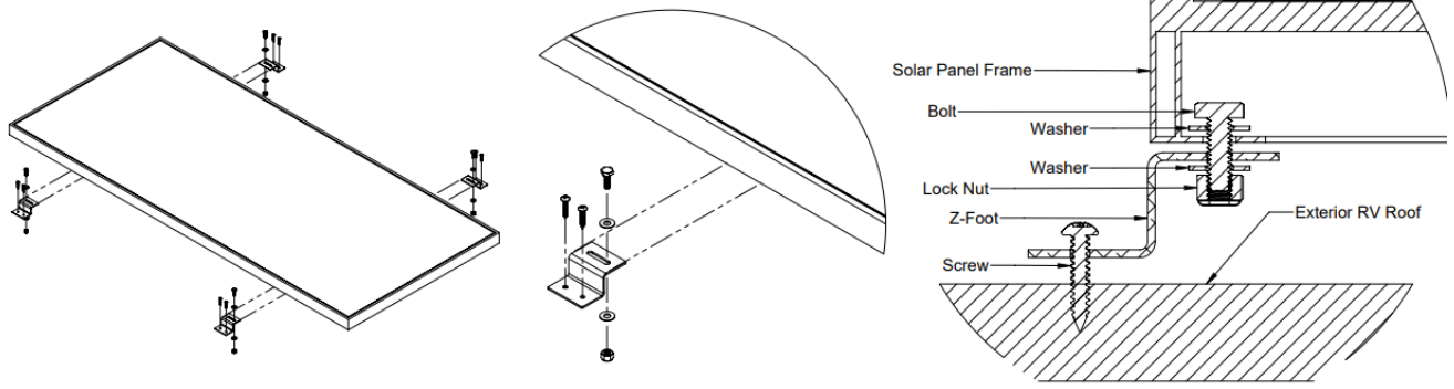
FIGURE 4-A: SOLAR PANEL INSTALLATION DETAILS
