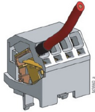
Cage clamp (PC/plugin cage clamp)
