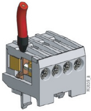
Screw terminal (PS/plugin screw)
