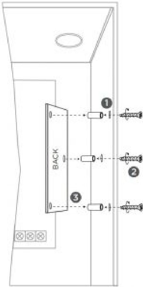
Figure 2: Standoff and Module Installation
