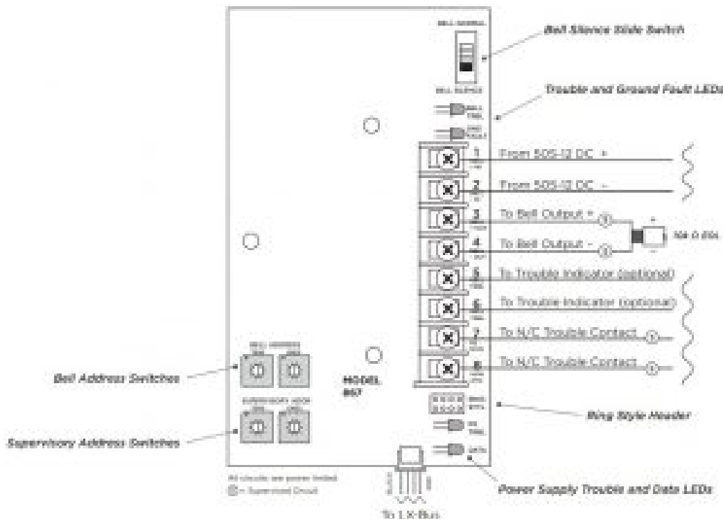
Figure 4: Wiring Connections
