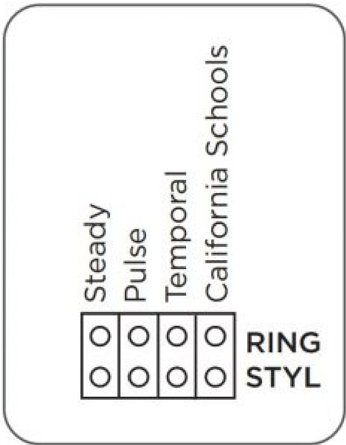
Figure 3: Ring Style Header Detail
