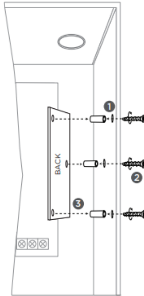
Figure 2: Standoff and Module Installation
