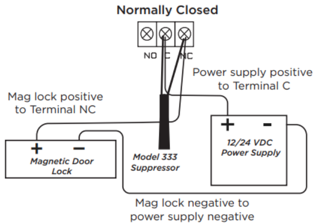
Figure 1: Typical Magnetic Lock Wiring
