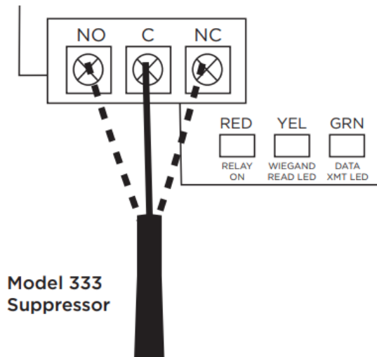
Figure 3: 333 Suppressor Installation on the 734
