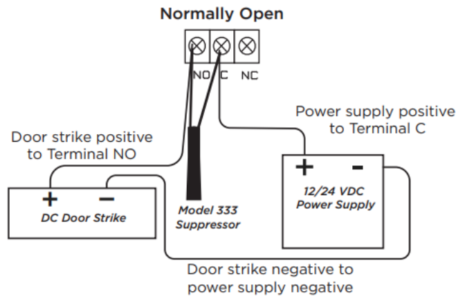
Figure 2: Typical Door Strike Wiring
