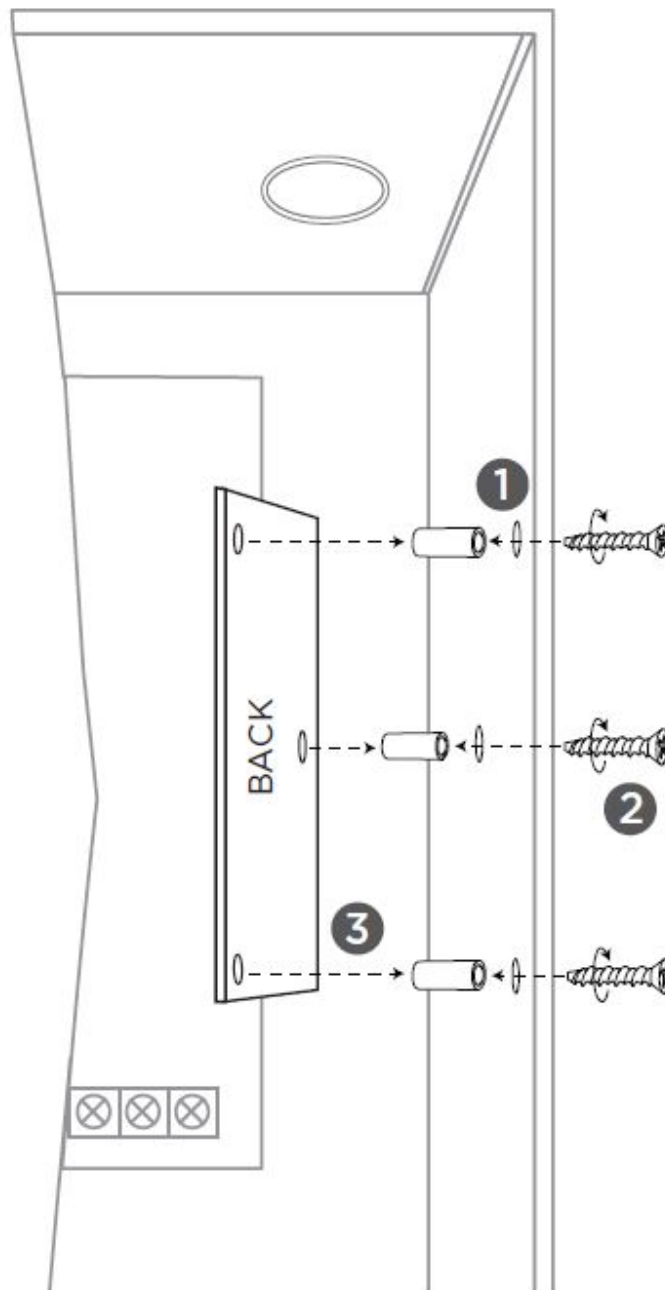
Figure 2: Standoff and Module Installation
