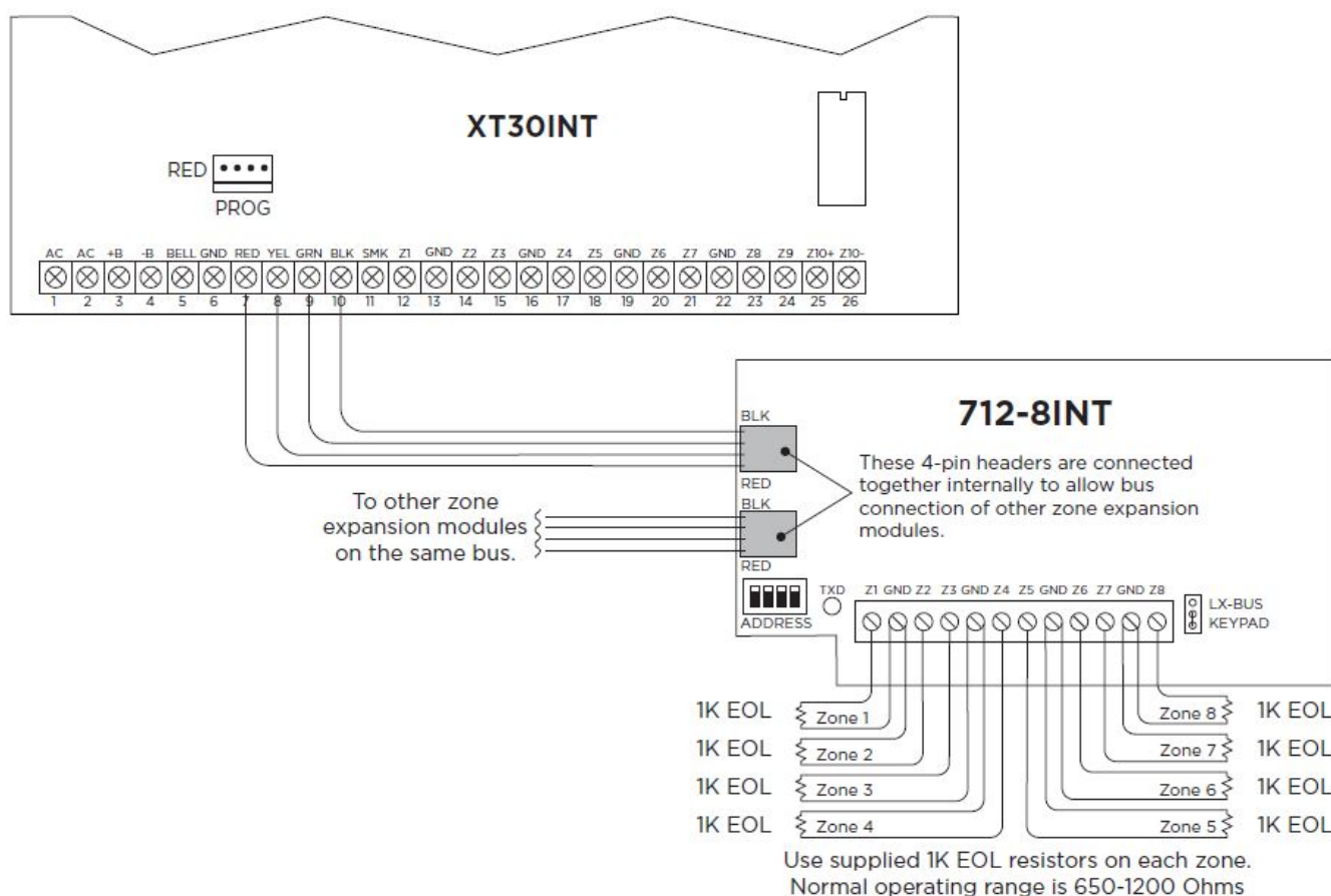
Figure 3: Wiring Diagram
