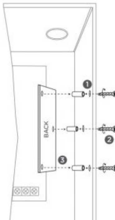
Figure 2: Standoff and Module Installation
