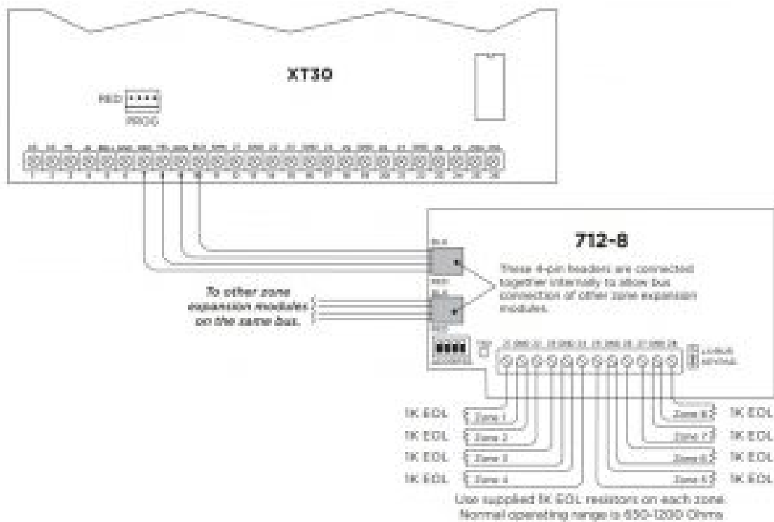
Figure 3: Wiring Diagram
