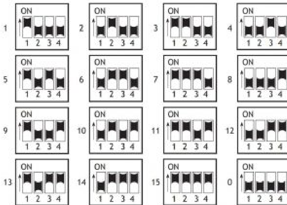
Figure 4: Addressing the Module
