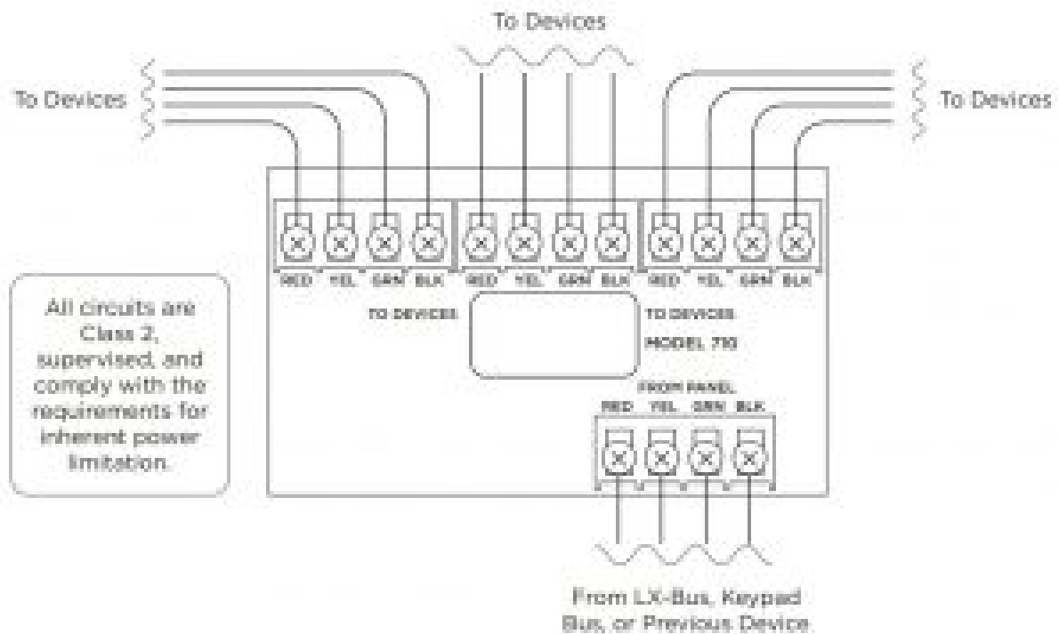
Figure 4: Module Wiring Diagram
