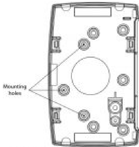
Figure 2: Mounting Hole Locations
