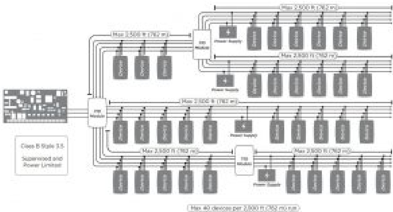
Figure 8: Wiring Multiple Circuits
