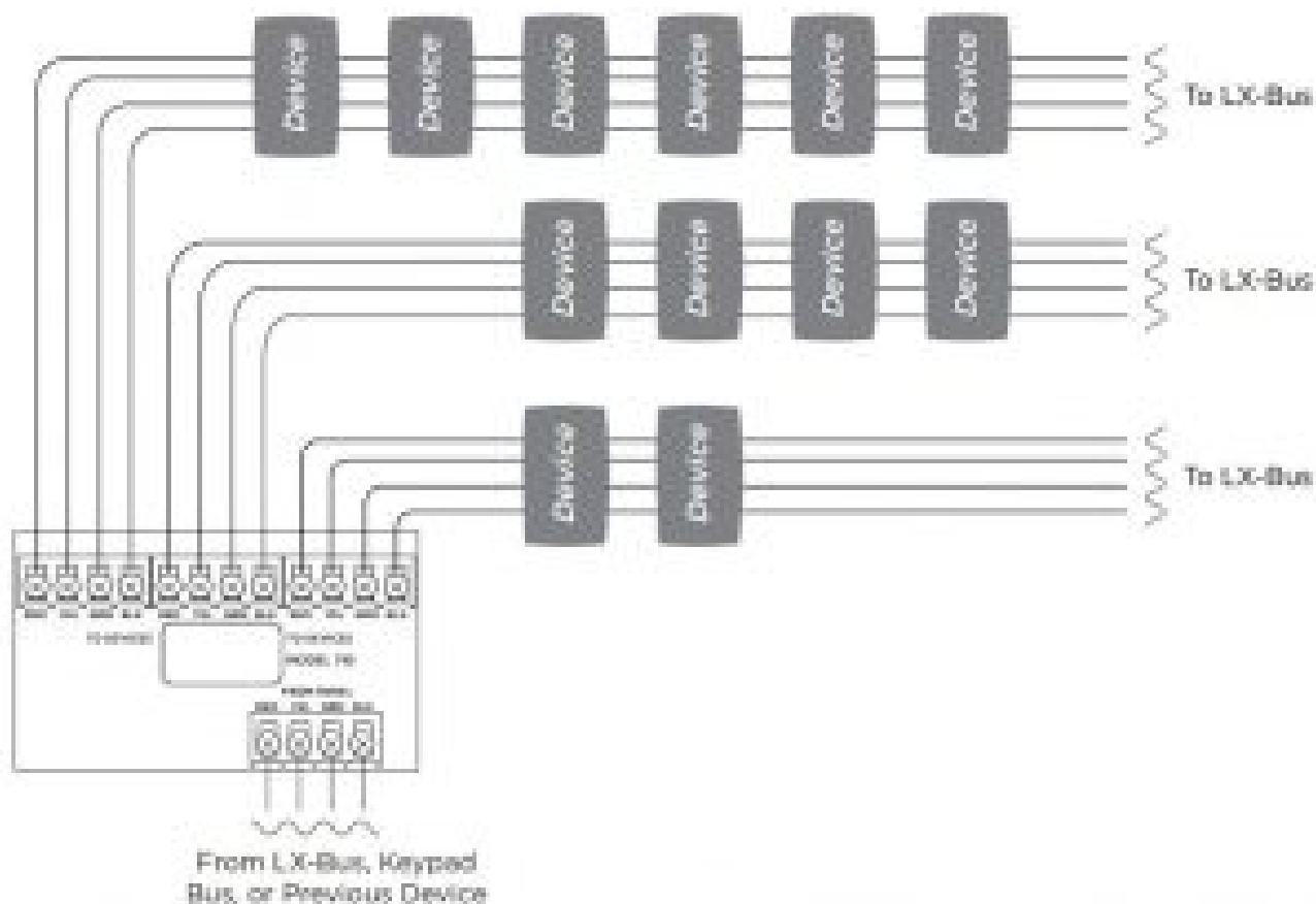
Figure 9: Using the Module as a Junction Box
