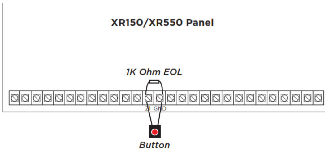
Figure 1: Button Placement
