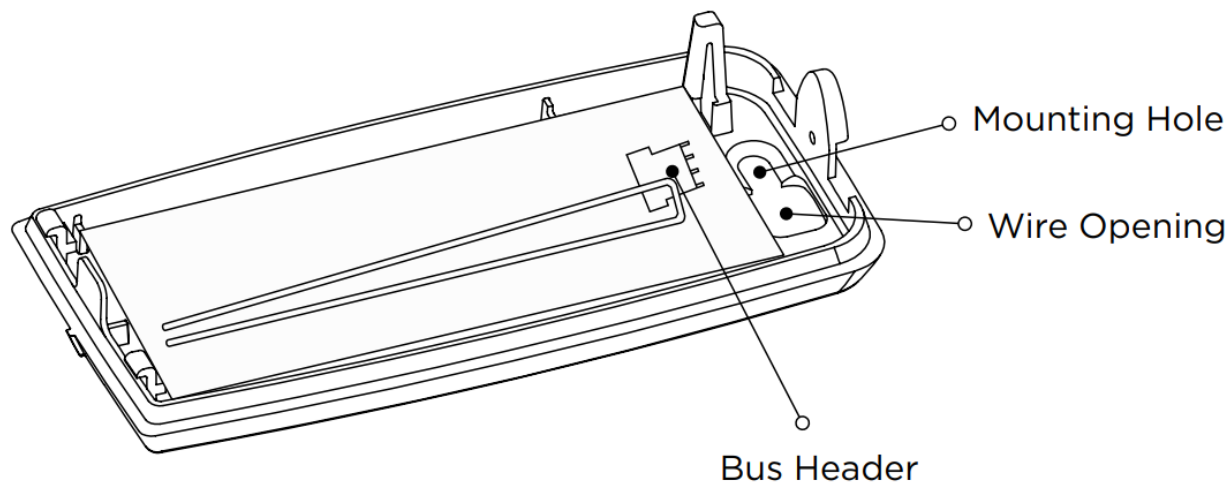
Figure 2: PCB and Mounting Holes
