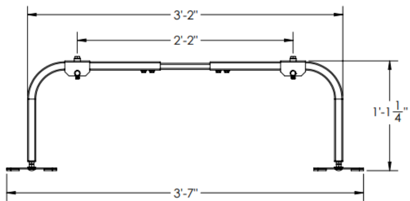
SIDE VIEW EXPANDED
