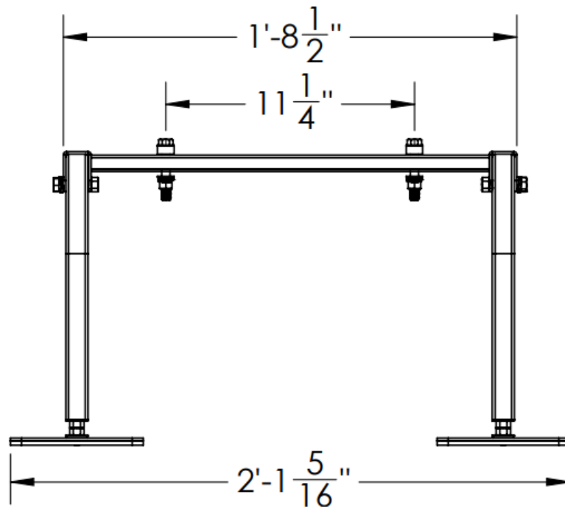
END VIEW RETRACTED
