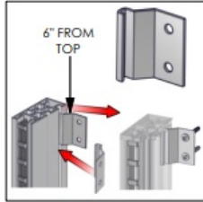
WALL MOUNT CLIPS
