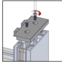
LOOSEN END CAP TO ATTACH TOP CROSS BRACE
