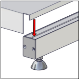
MFY-36-17-BASE-PAN
