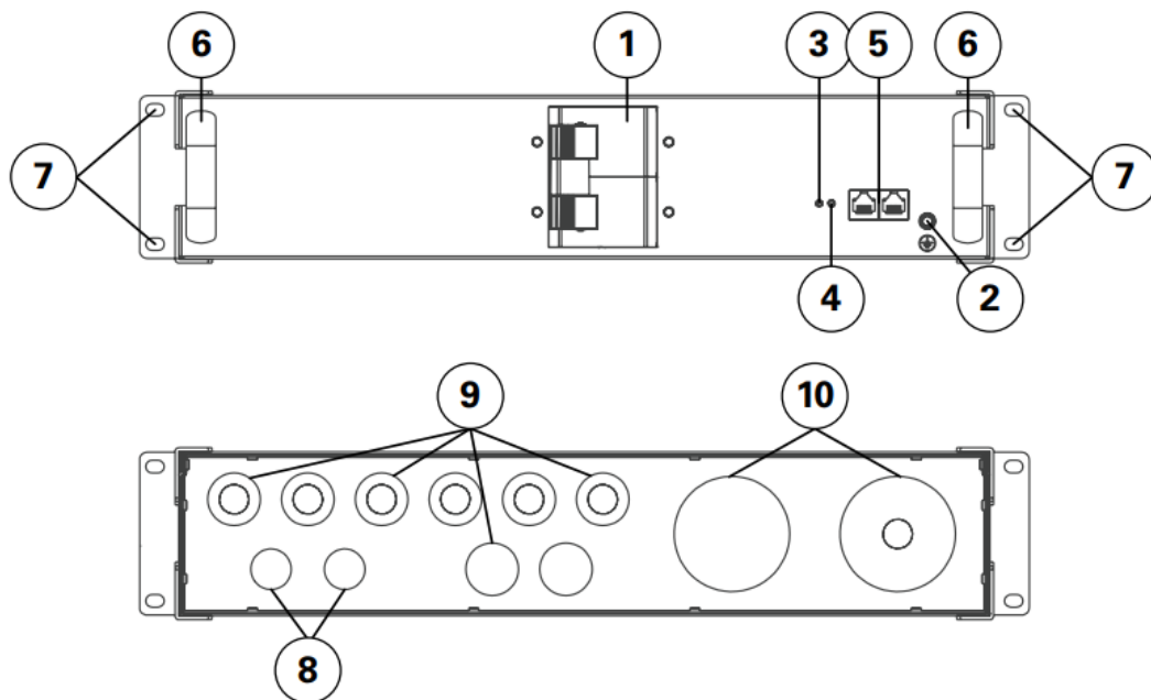
Figure 2. Battery Module Combiner (front, back)
