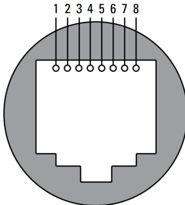
Figure 4. LYNK Port Communication RJ45 pin assignment
