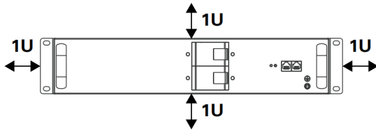
Figure 9. Spacing around the Battery Module Combiner
