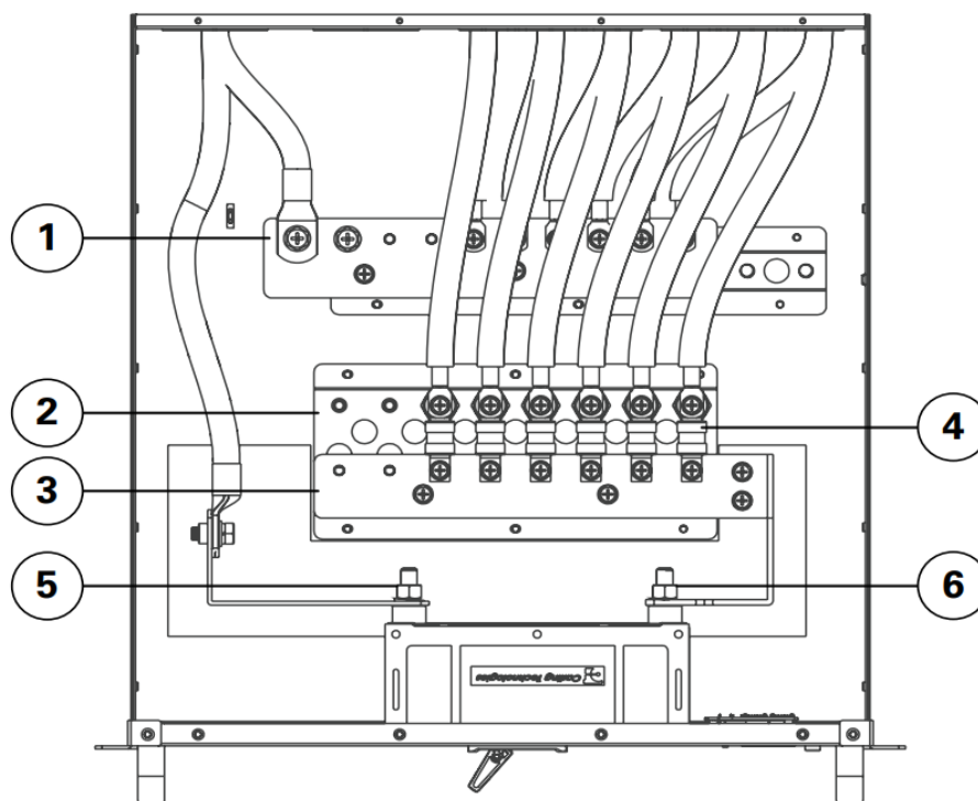
Figure 6. Battery Module Combiner with the top removed
