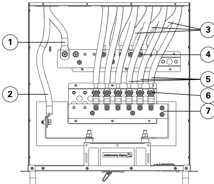
Figure 7. Battery Module Combiner Cable Connections
