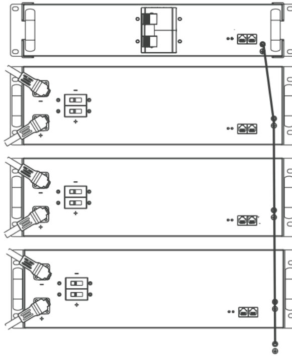
Figure 12. Grounding the Battery Module Combiner
