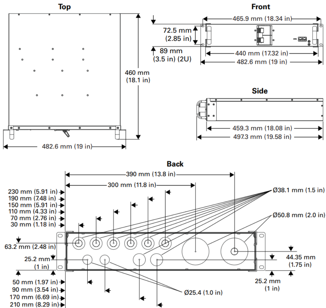
Figure 1. Battery Module Combiner Dimensional Drawings
