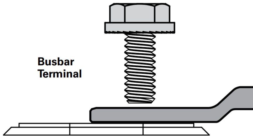
Figure 5. Busbar Terminal Installation
