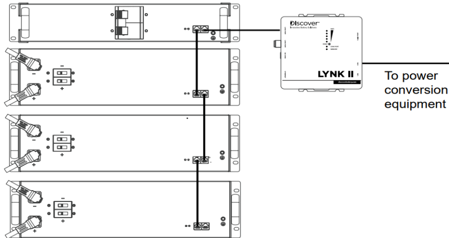
Figure 3. Battery Module Combiner connected to the Battery Module Network and a LYNK II Gateway
