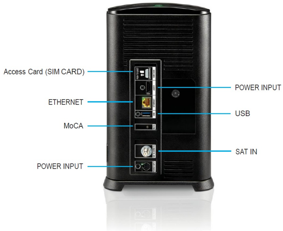
FIGURE 3: Genie 2 REAR PANEL
