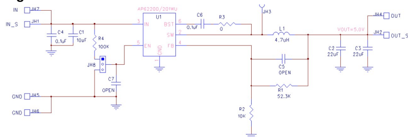
Figure 3. AP62200WU-EVM Schematic
