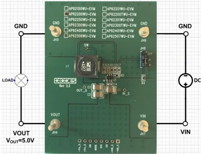
Figure 2. AP62200WU-EVM
