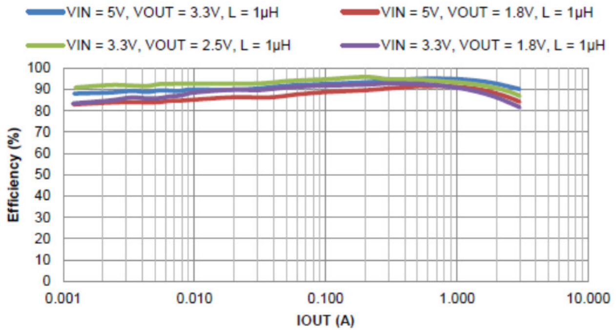
Figure 6. PFM Efficiency vs. Output Current
