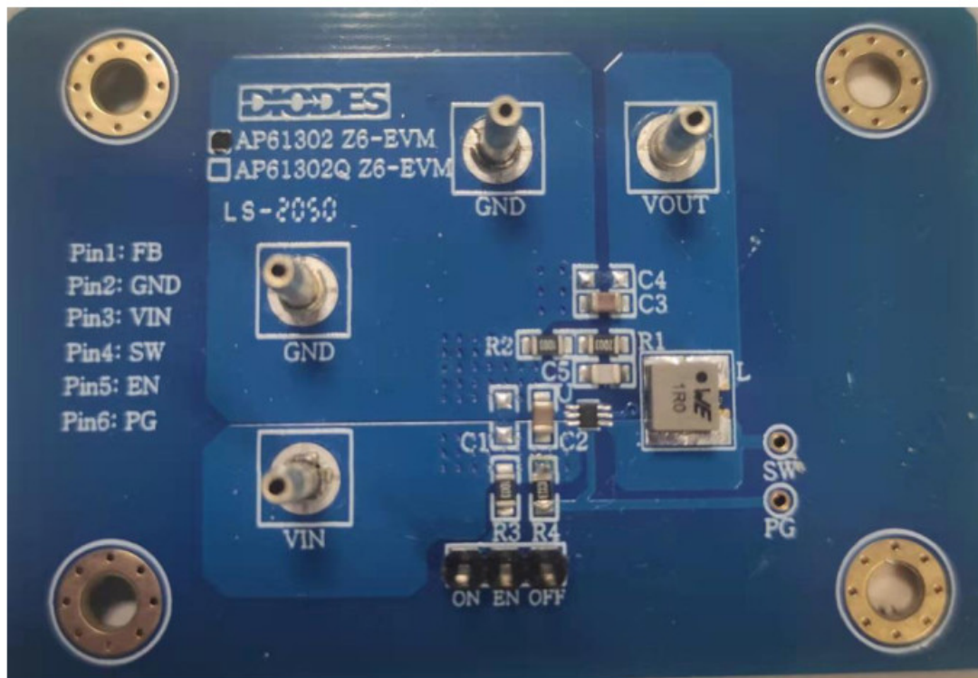
Figure 5. AP61302Z6 EV Board View
