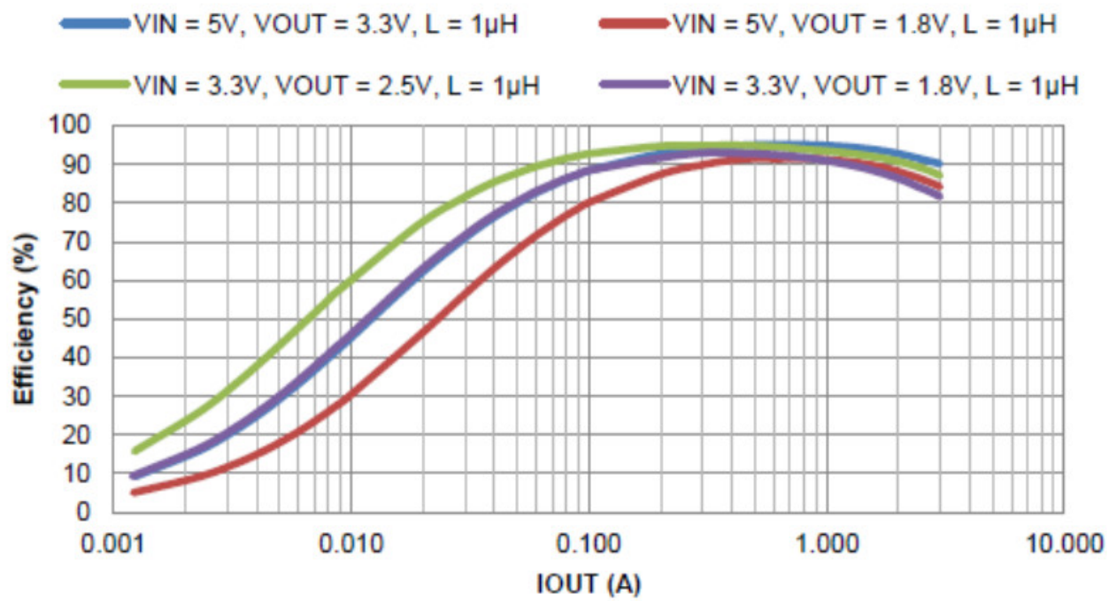
Figure 7. PWM Efficiency vs. Output Current
