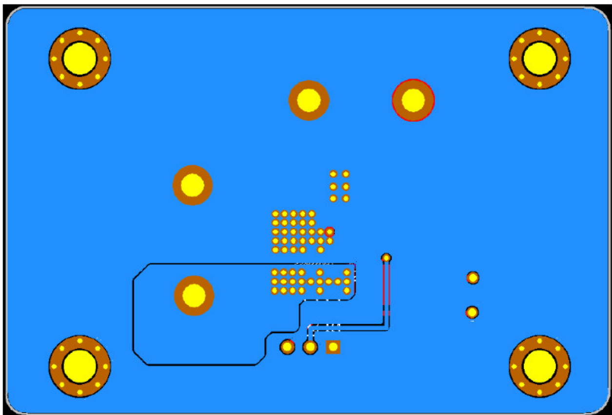
Figure 4. AP61302Z6 - EVM - Bottom Layer
