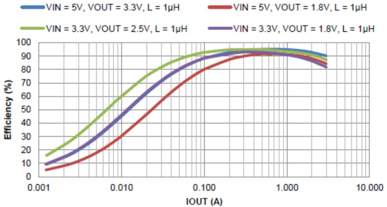
Figure 7. PWM Efficiency vs. Output Current
