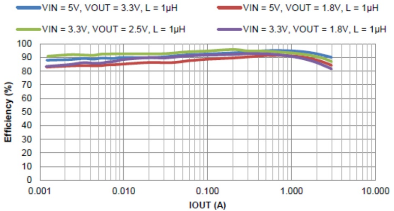
Figure 6. PFM Efficiency vs. Output Current
