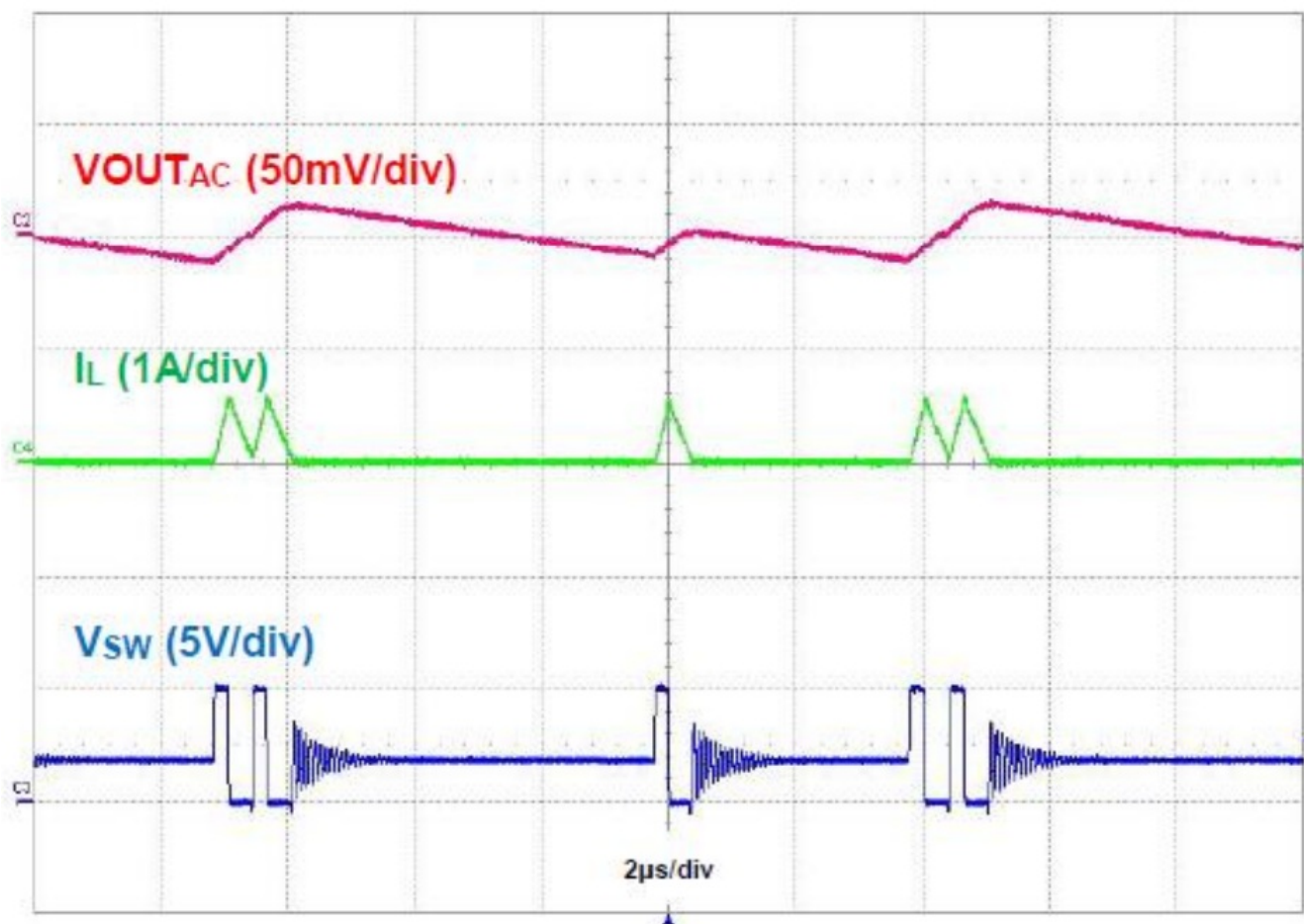
Figure 8. Output Voltage Ripple, IOUT = 50mA
