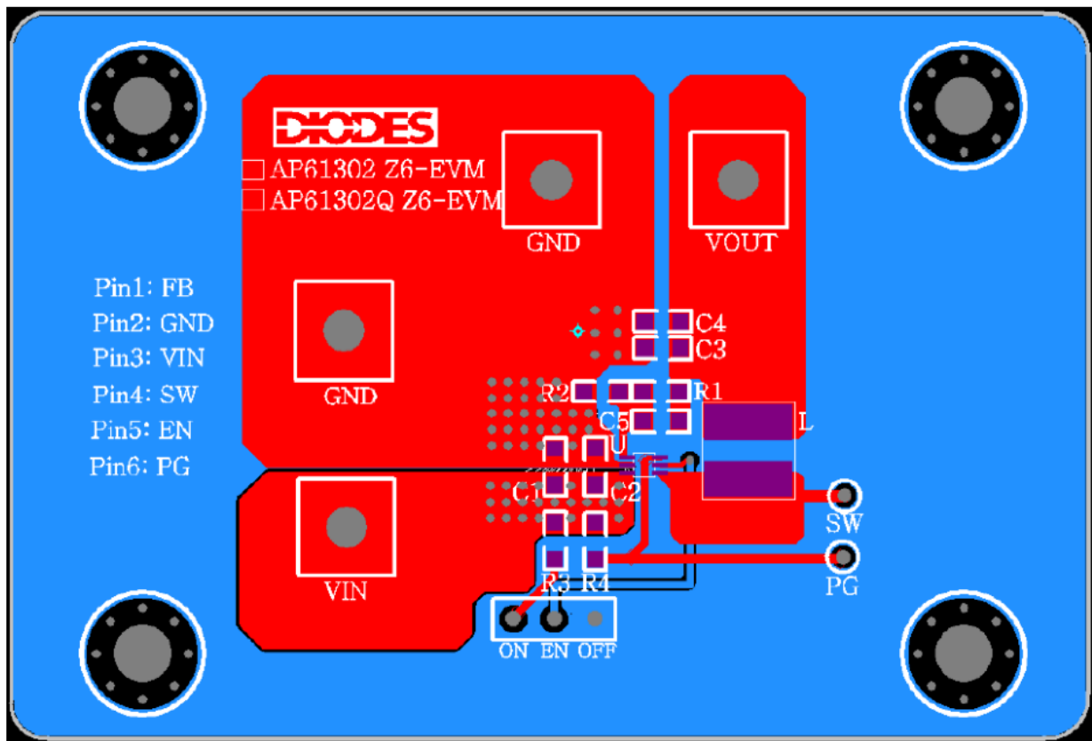
Figure 3. AP61302QZ6 - EVM - Top Layer
