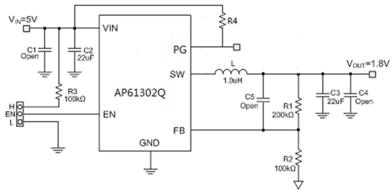
Figure 2. Typical Application Circuit
