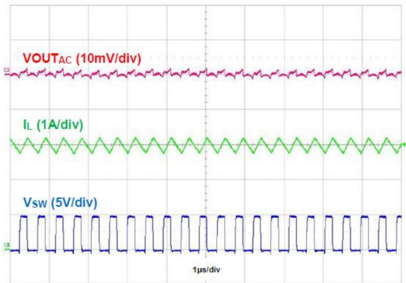
Figure 9. Output Voltage Ripple, IOUT = 1A
