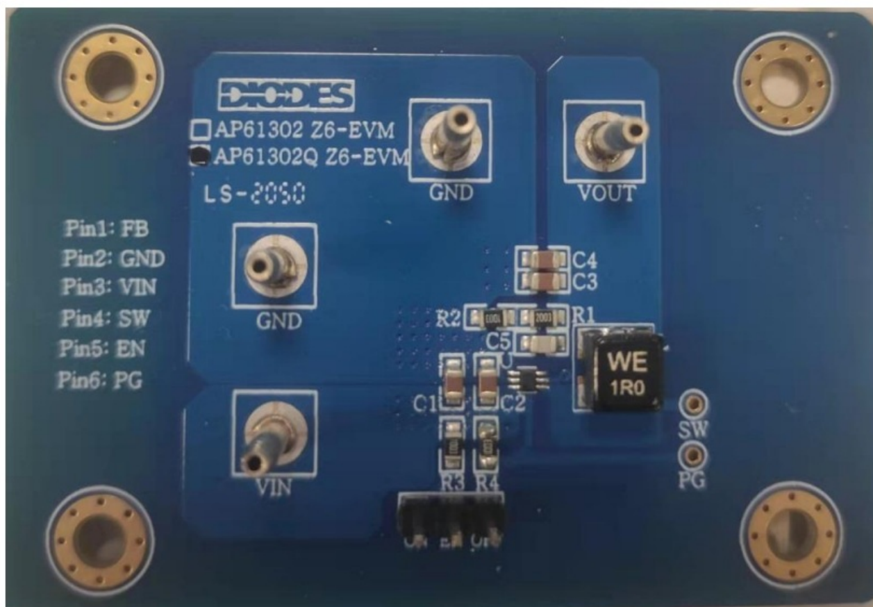
Figure 5. AP61302QZ6 EV Board View
