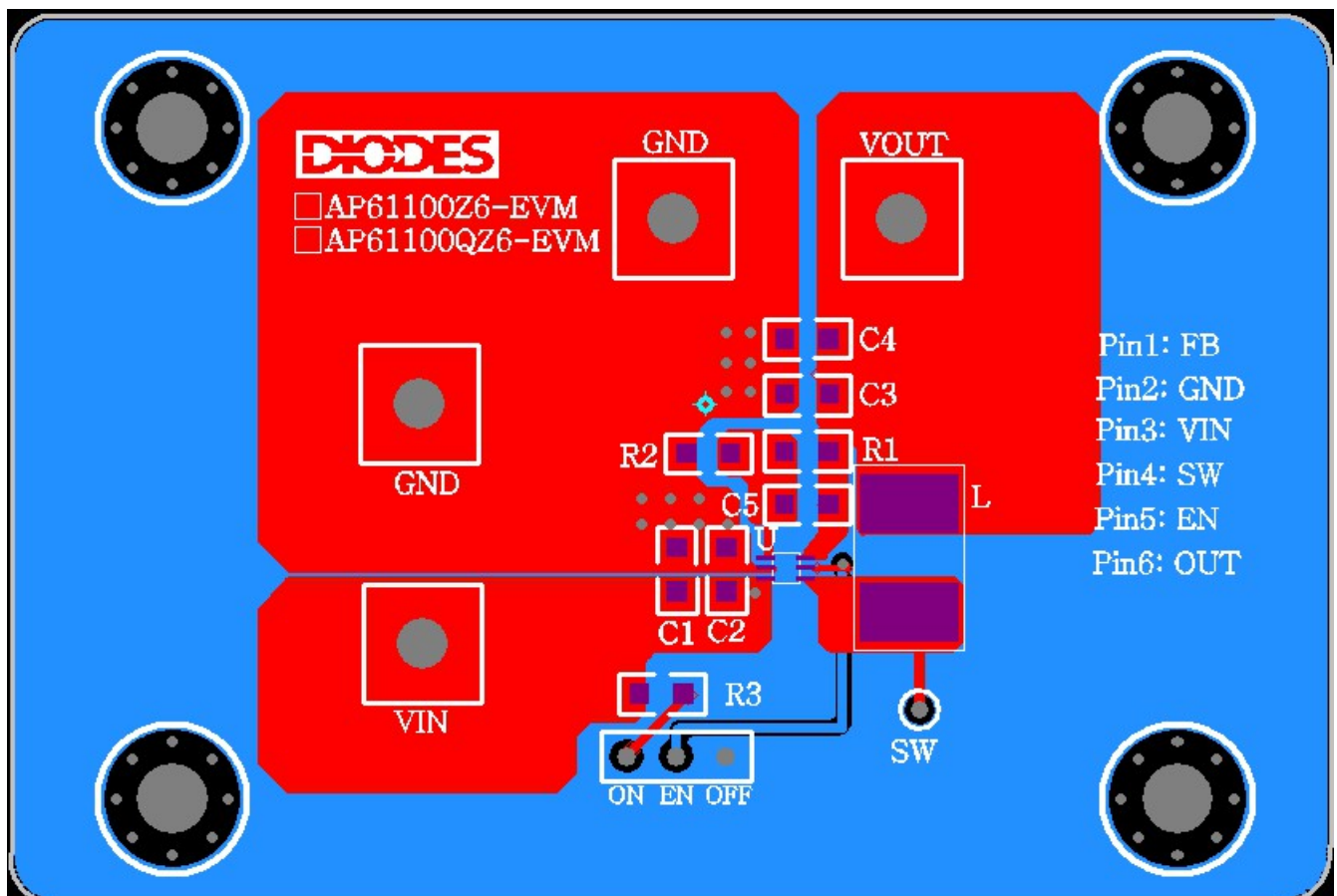
Figure 3. AP61100Z6 – EVM – Top Layer
