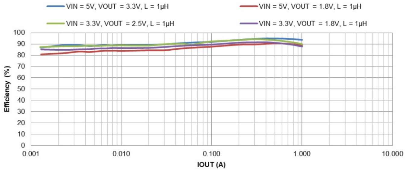
Figure 6. PFM Efficiency vs. Output Current
