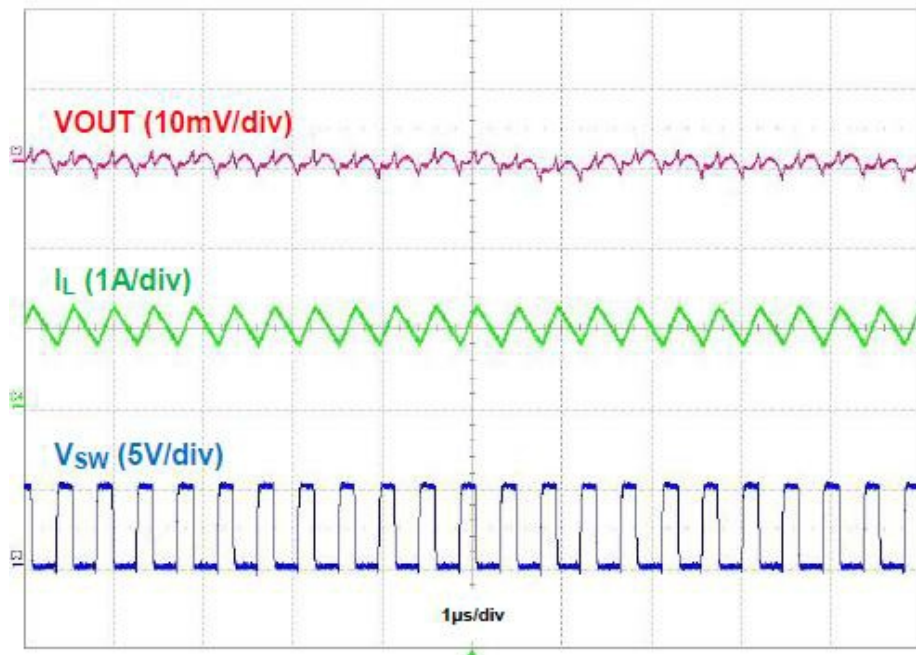
Figure 9. Output Voltage Ripple, I_{OUT} = 1\text{A}
