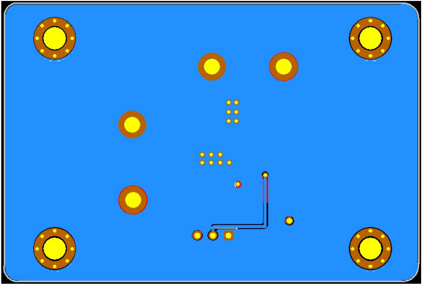
Figure 4. AP61100Z6 – EVM – Bottom Layer
