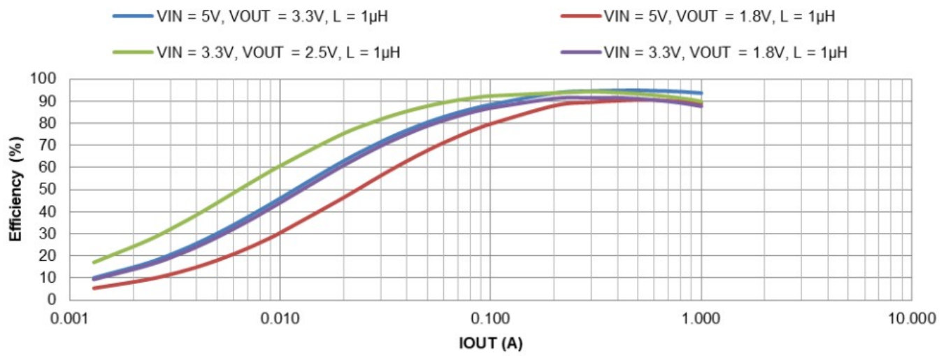
Figure 7. PWM Efficiency vs. Output Current
