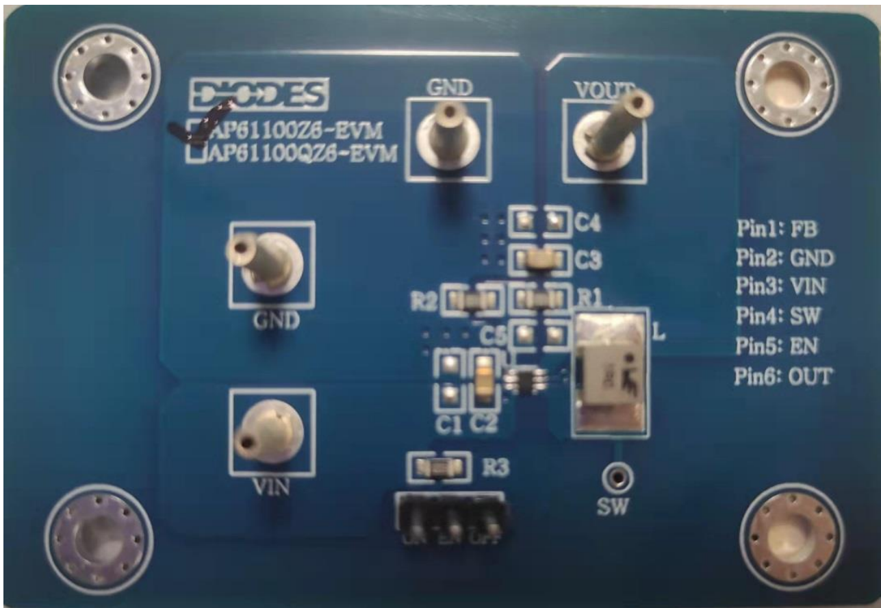
Figure 5. AP61100Z6 EV Board View
