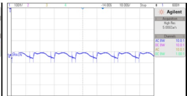
Figure:17 5V Ripple at 230Vac at FL
