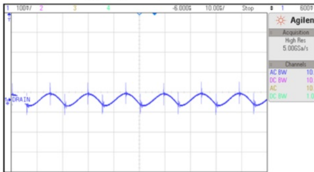
Figure:14 12V Ripple at 115Vac at FL .
