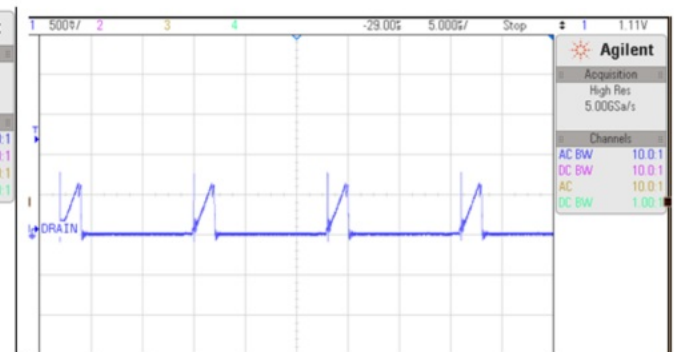
Fig:11 V_{cs} at 264V Acin at FL
