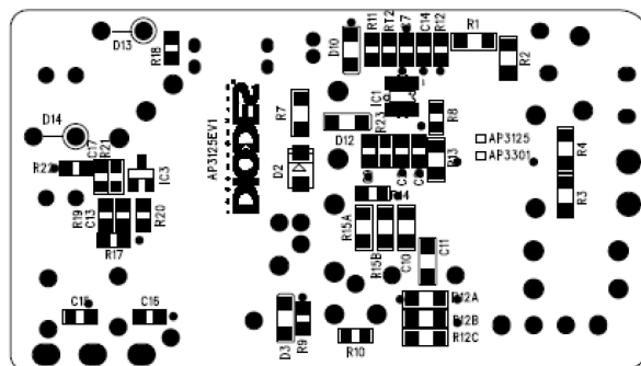
Figure 5: PCB Board Layout Bottom View
