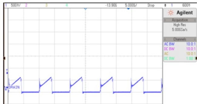
Fig:9 V_{cs} at 90V Acin at FL
