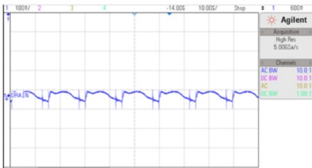
Figure:16 5Vo Ripple at 115Vac at FL
