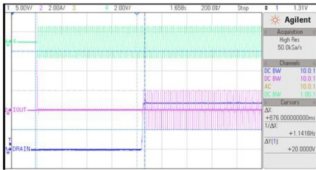
Fig:12 Turn on VAC_in, IAC_in, 12Vo at 115Vac at FL
