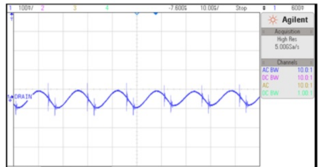
Figure:15 12V Ripple at 230Vac at FL
