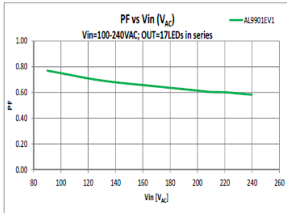
Figure 3. PFC vs. Vin
