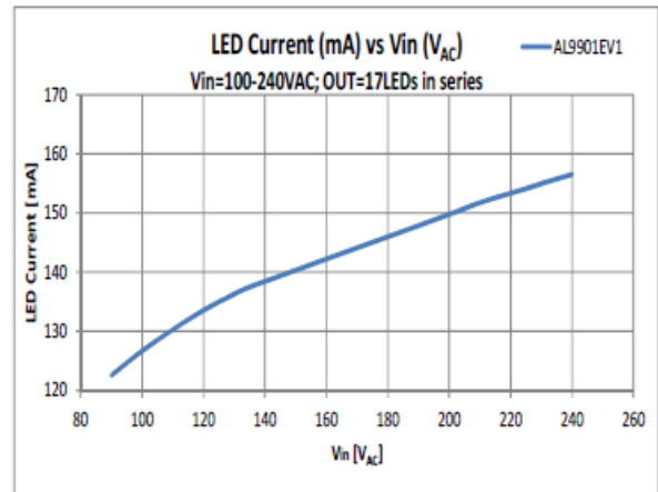
Figure 2. LED Current vs. Vin
