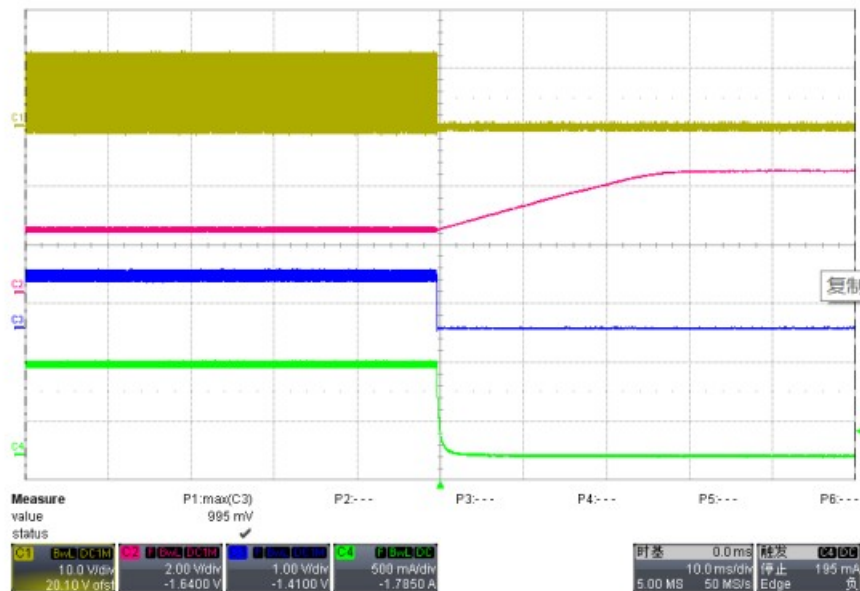
Figure 10. VOUT Short to GND Protection with 100% Duty
