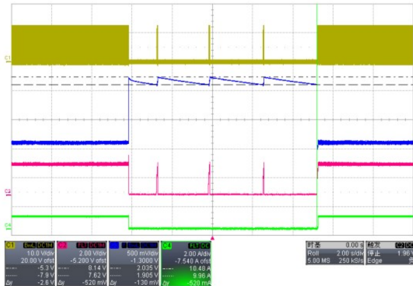
Figure 8. LED Open Protection with 100% Duty
