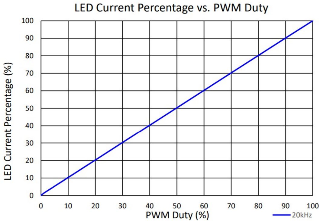
Figure 7. LED Current Percentage vs. PWM Duty
