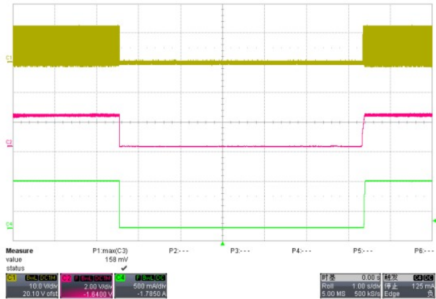
Figure 11. Overtemperature Protection with 100% Duty
