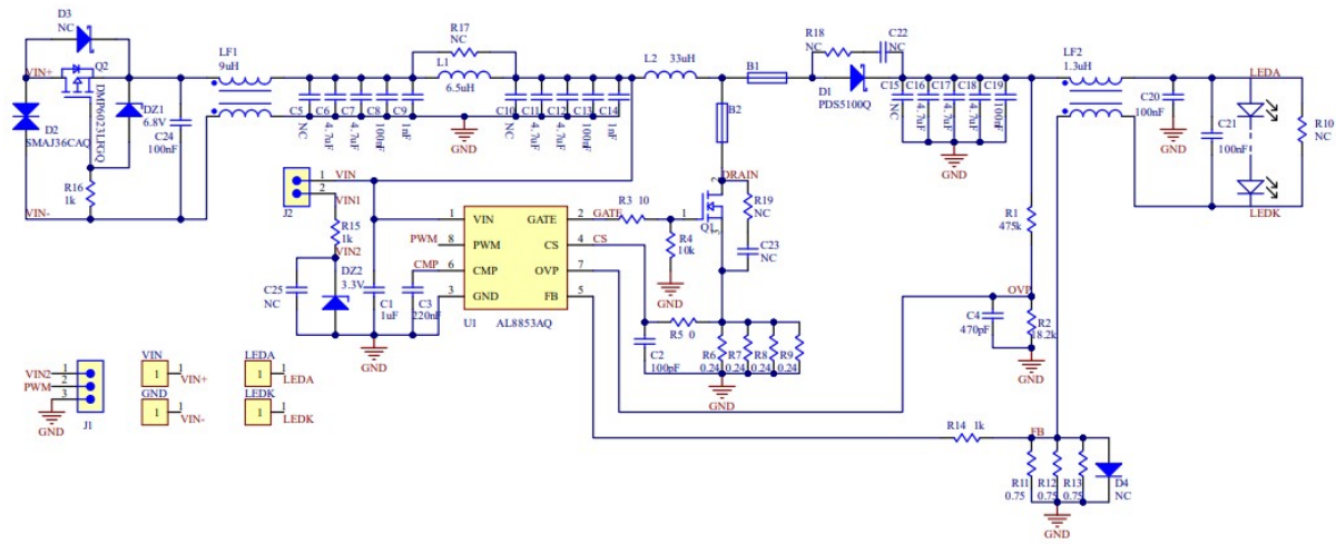
Figure 5. Schematic Circuit
