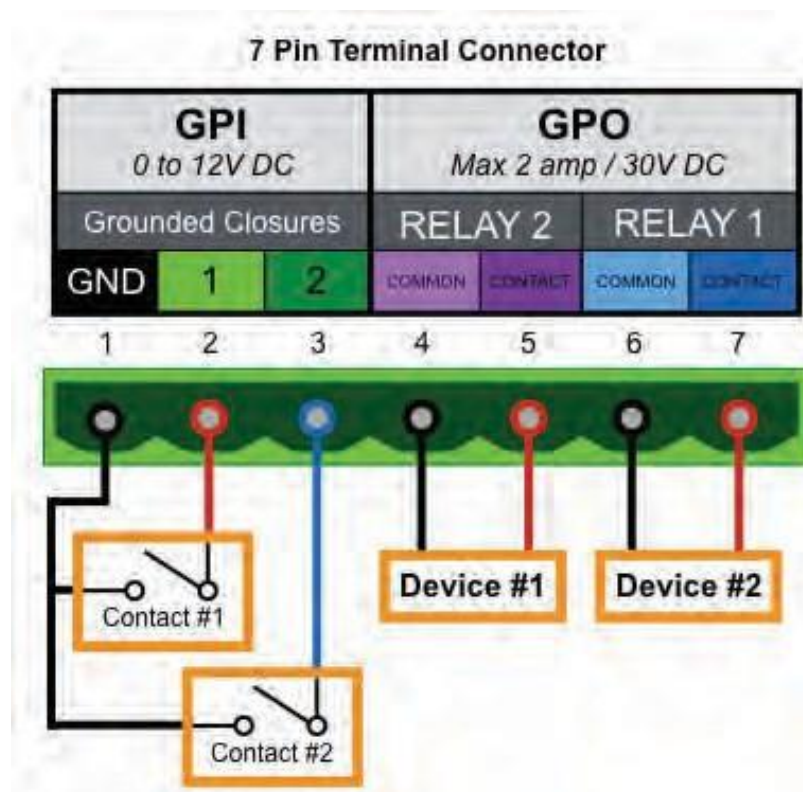
GPIO Terminal Connector
