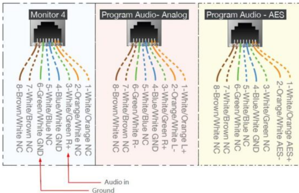
Connection diagrams for EAS Monitor Input 4 (DAS3-EX/GX), Analog and AES Program Audio.
