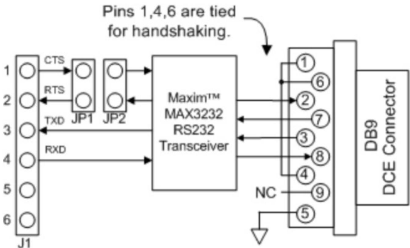
Figure 1. PmodRS232 block diagram.
