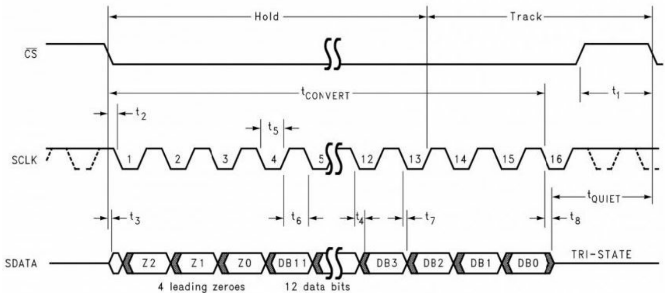
Figure 1. Timing diagram.
