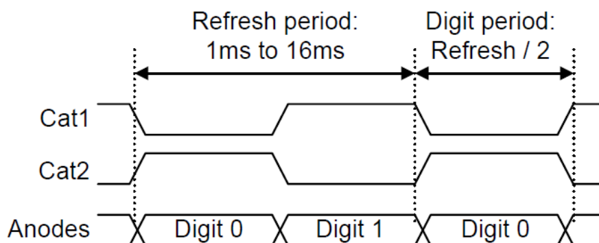
Figure 15. Display drivers.
