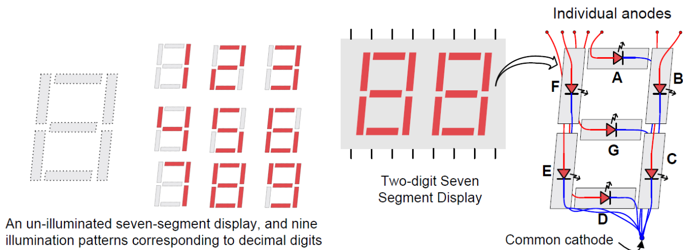
Figure 14. Seven-segment displays.
