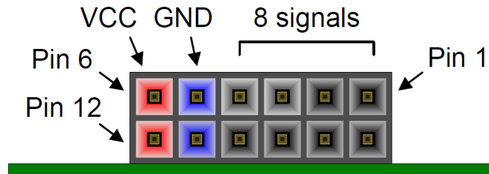
Figure 16. Pmod ports – front view as loaded on PCB.
