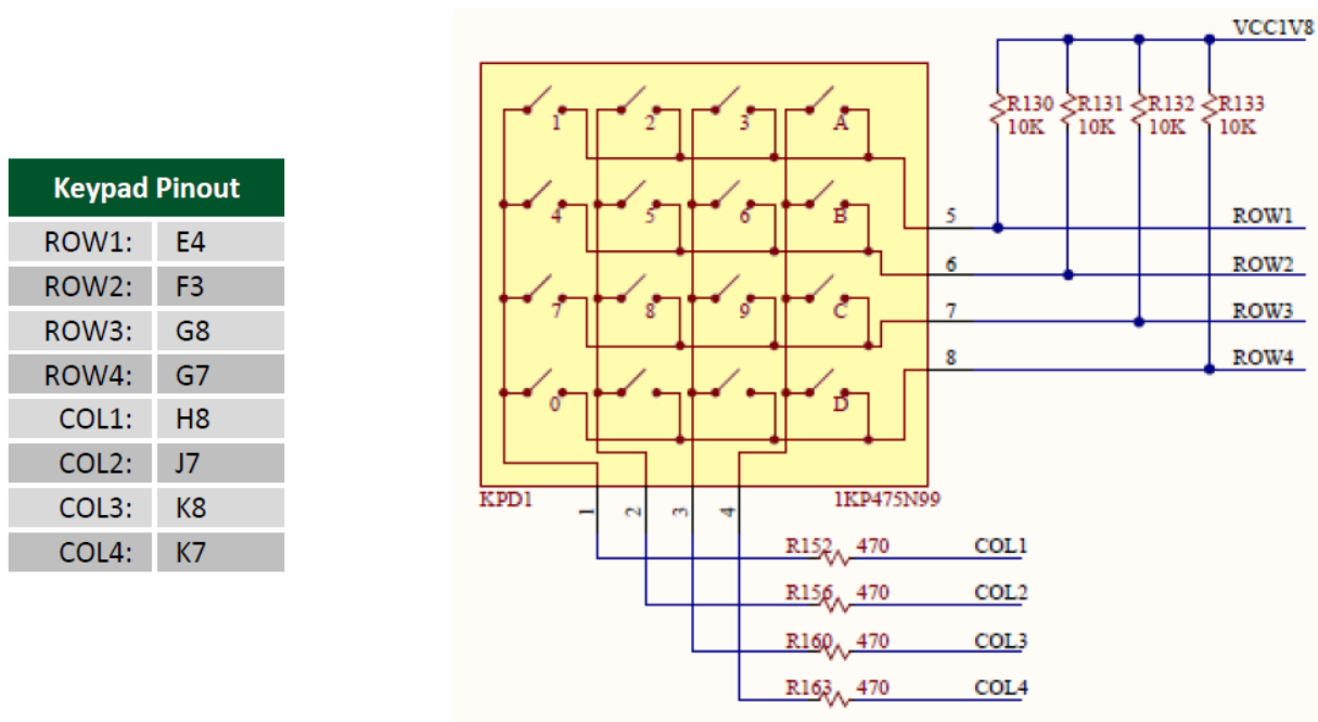
Figure 13. Keypad schematic
