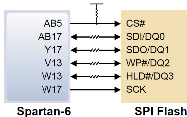
Figure 1. SPI flash interface.
