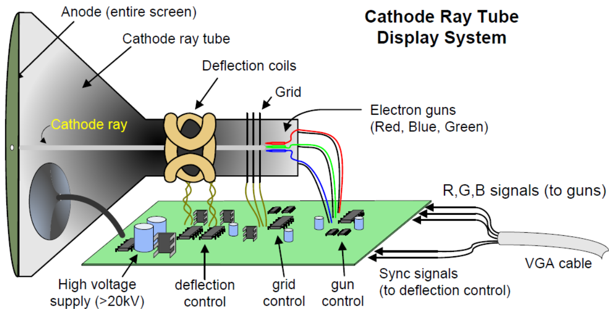
Figure 4. Cathode ray tube display system.
