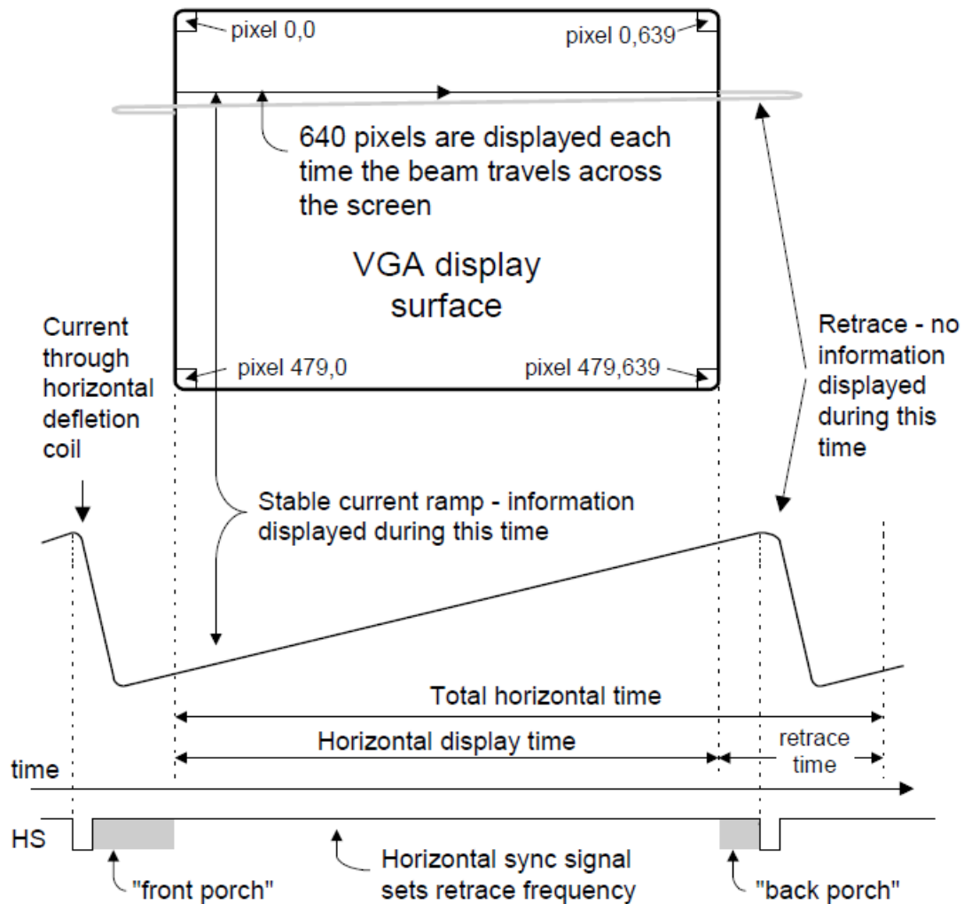
Figure 5. VGA horizontal synchronization.
