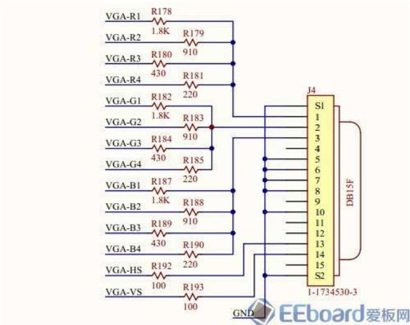
Figure 2. VGA interface.
