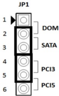
Figure 3: Jumper Block JP1
