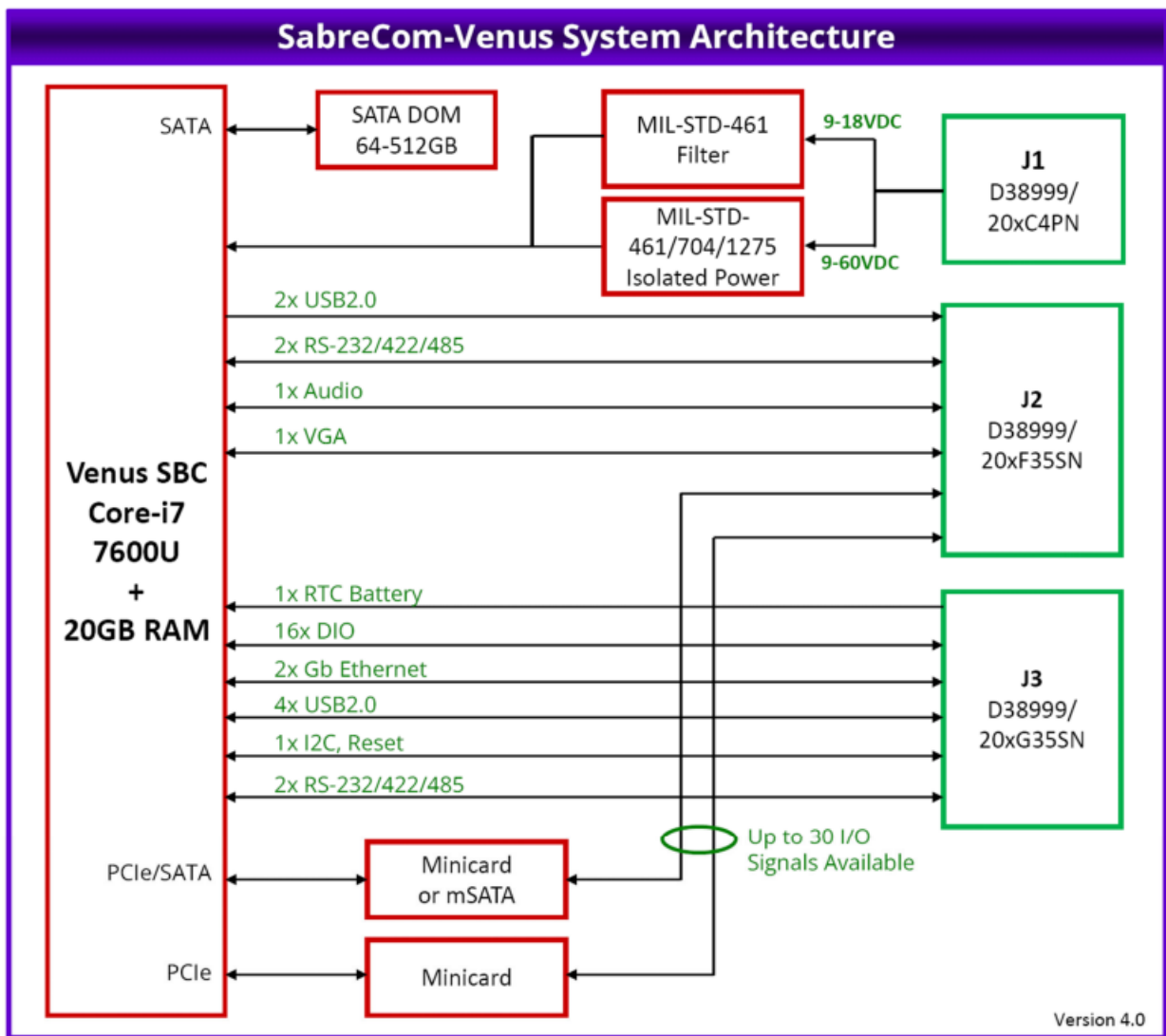
Figure 1: System Architecture of SabreCom-VNS
