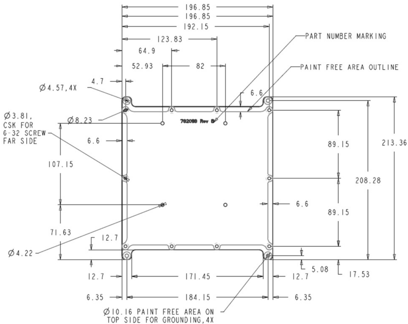
Bottom plate dimensions showing mounting hole locations
