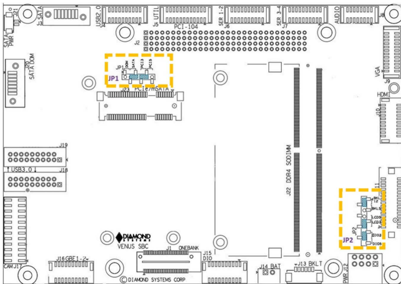
Figure 2: Jumper Blocks on Venus Carrier Board
