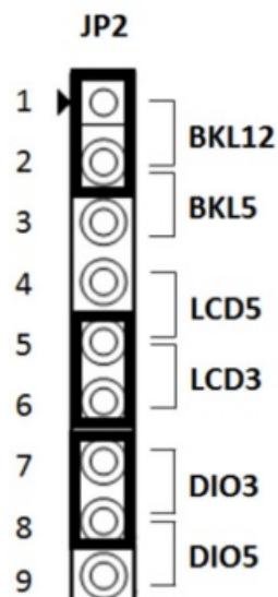
Figure 4: Jumper Block JP2
