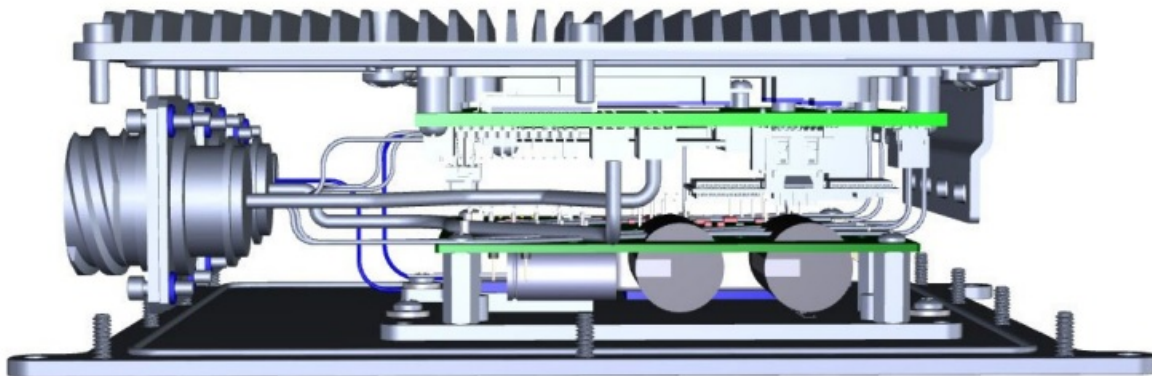
3d side view showing JMM-7500 power supply mounted to bottom cover (flat exterior surface) and VNS776KL-xGD SBC mounted to the top cover (with heat sink fins).
