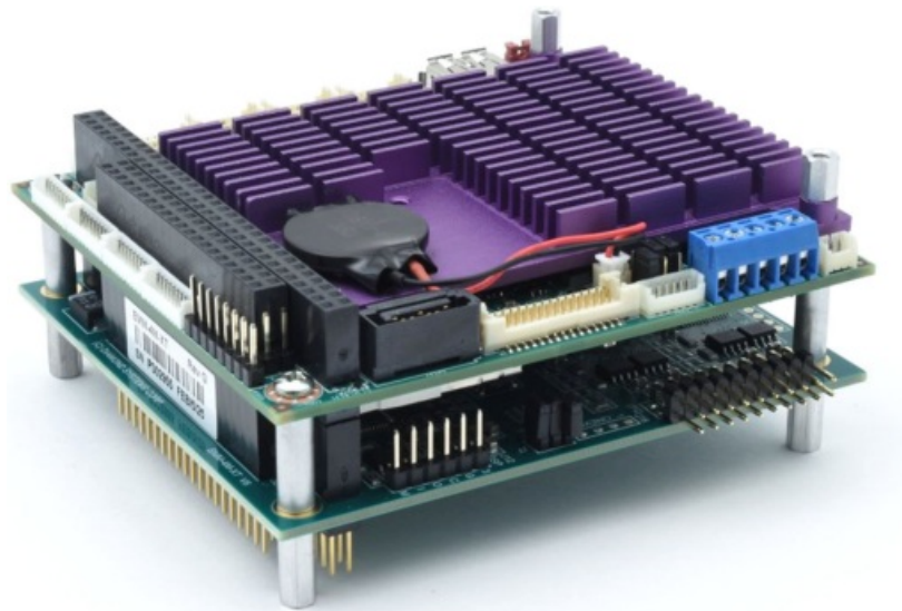
Figure 1-3: Samson with PC/104 I/O module installed underneath
