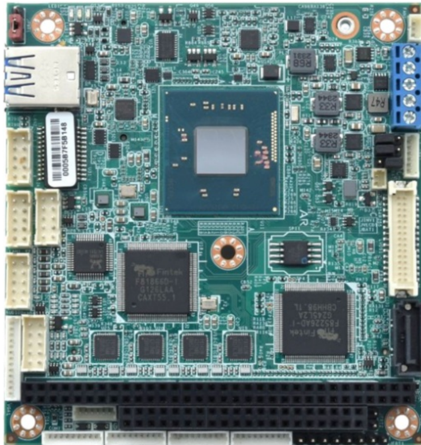
Figure 1-1: SAMSON PC/104 SBC – Top View
