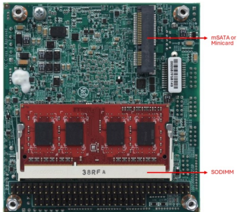
Figure 5-2: Bottom view showing mSATA/Minicard and SODIMM sockets
