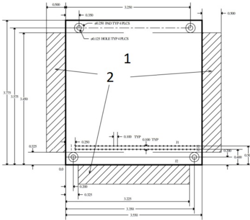
Figure 4-1: Samson PC/104 board dimensions – primary side
