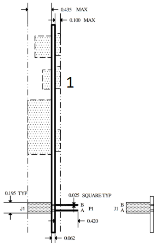
Figure 4-2: Samson PC/104 board dimensions – secondary side
