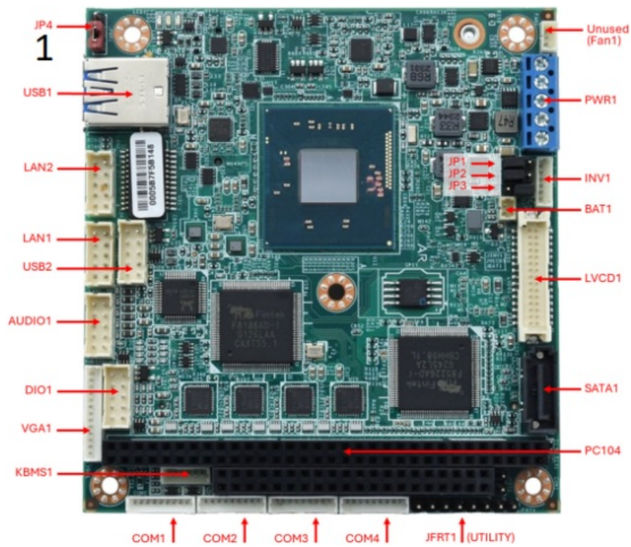
Figure 5-1: Top view (heat sink omitted)
