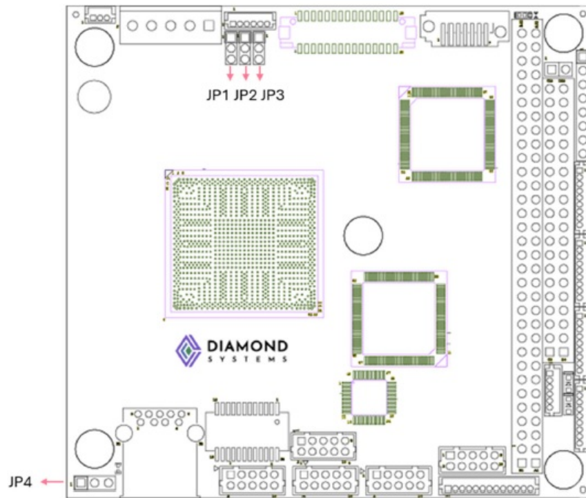
Figure 4: Default Jumper Locations
