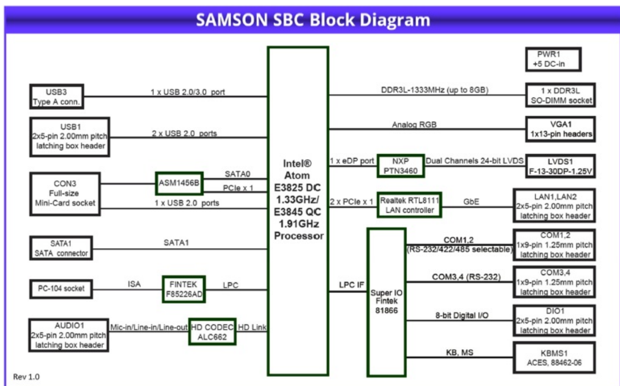
Figure 1: SAMSON PC/104 CPU Module Block Diagram
