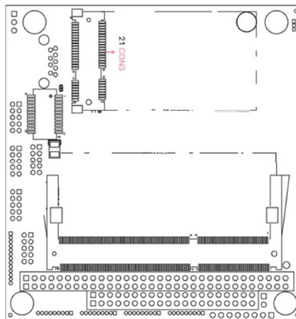
Figure 2: Top view (heat sink omitted)
