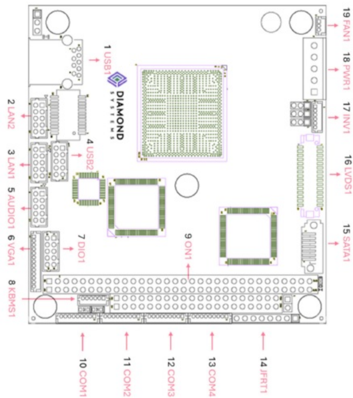
Figure 2: Top view (heat sink omitted)
