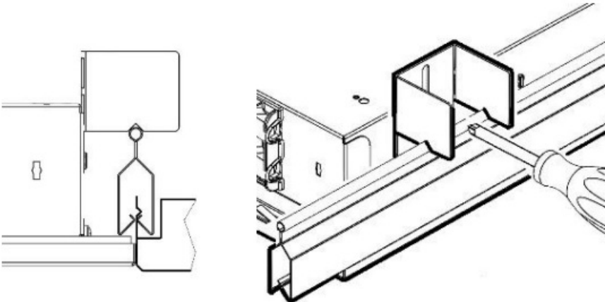
8. Electrical connection is made via integrated connection back-flap – allows for LEN L1 (emergency) and D1/D2 where specified.
