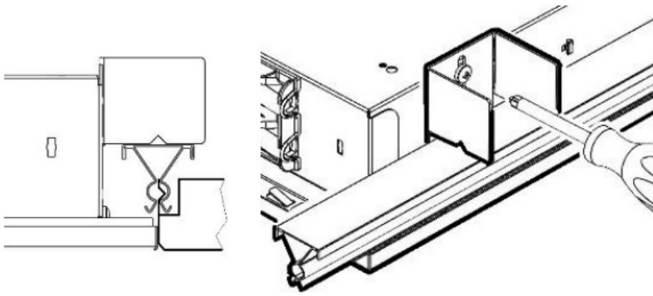
7. SAS 150 clip-in, fixture stops up against concealed T bar
