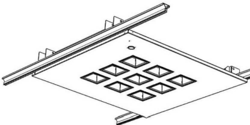
9. Installed fixture on SAS 120 grid (Sensored / Emergency version shown)
