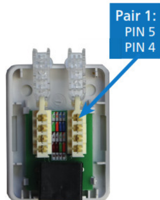
Toolless Cat RJ45 termination box
