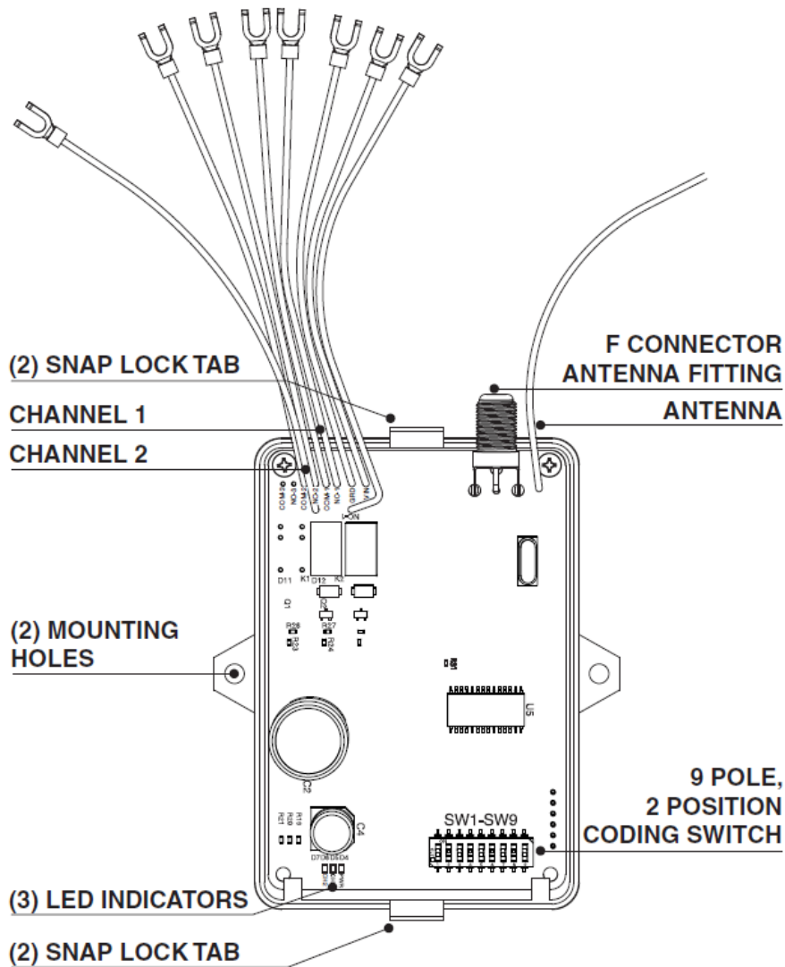
IMAGE 3: RECEIVER BASE DETAIL
