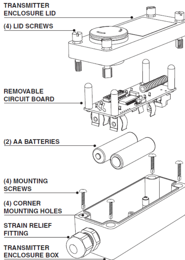
IMAGE 4: TRANSMITTER ASSEMBLY
