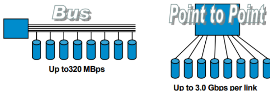
Figure 1: Parallel U320 SCSI bus versus point to point Serial Attached SCSI connection
