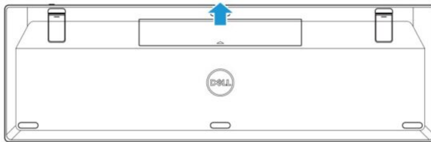
Figure 18. Removing the battery cover
