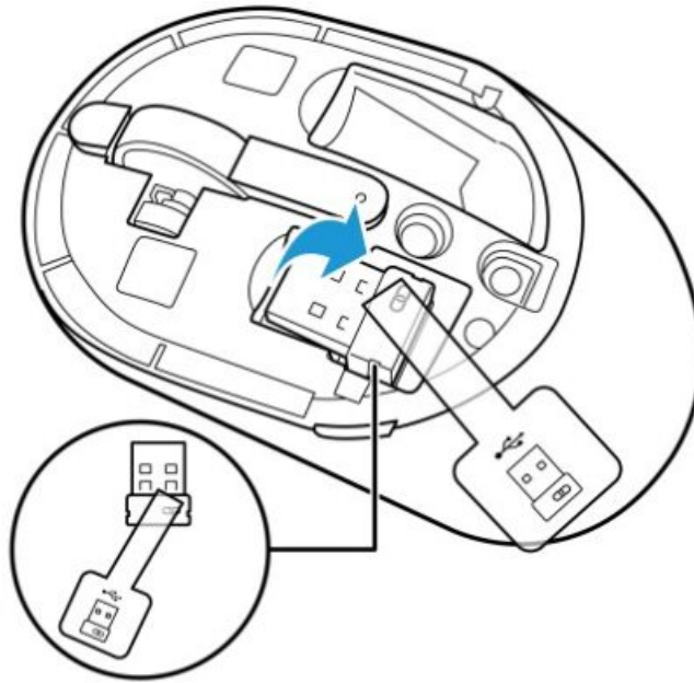
Figure 4. Removing the Dell Secure Link USB Receiver
