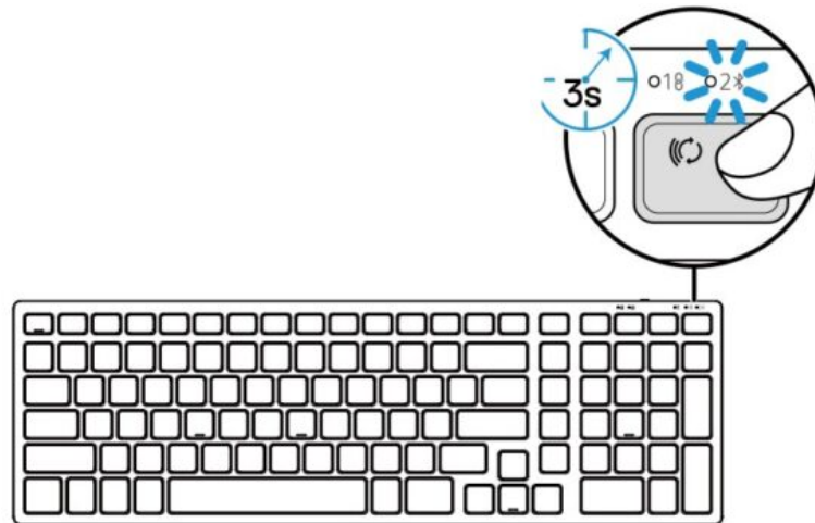
Figure 26. Initiating the Bluetooth pairing mode
