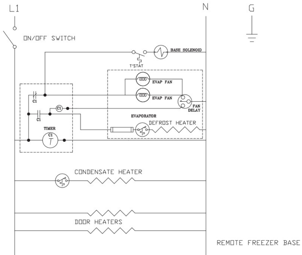
Wiring Diagram, F18PD
