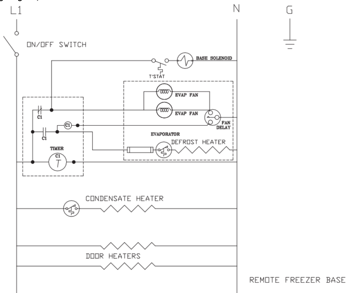
Wiring Diagram, F18PD
