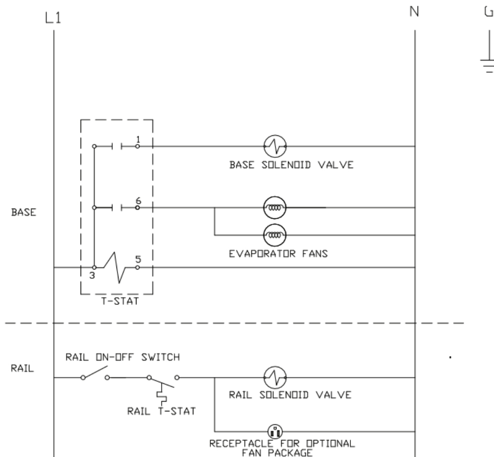
Remote reef with mech cooled rail Wiring Diagram, F18FC
