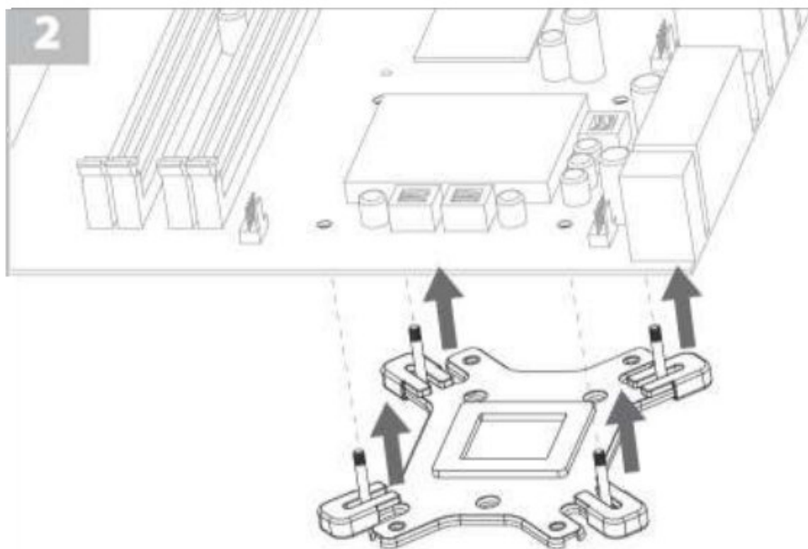
Back plate installation (Intel)
