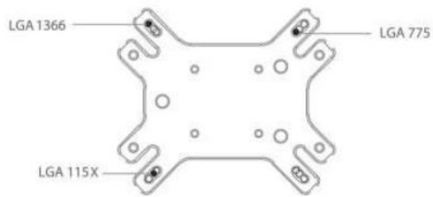
Back plate installation (Intel)
