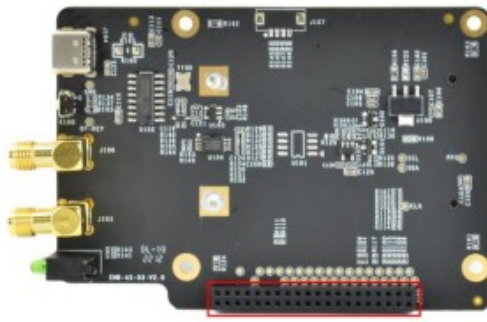
Figure 10 Female header of DEBIX LoRa board
