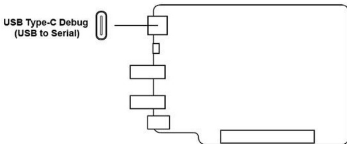
Figure 3 Debug interface
