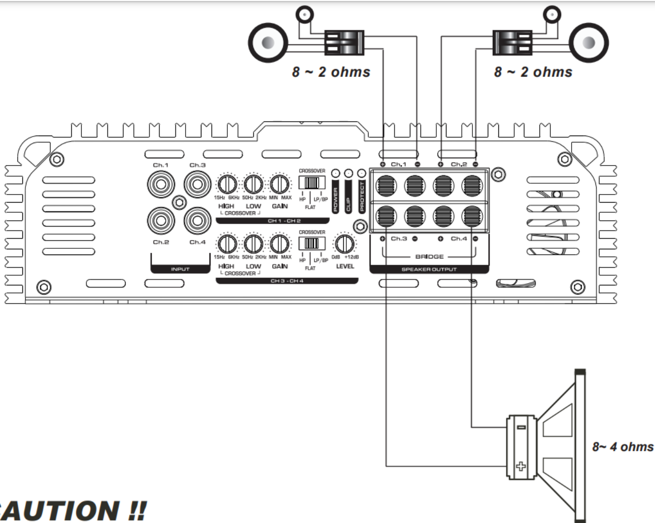
3-4D. WDX PRO 4 CHANNEL AMPLIFIERS' SPEAKER CONNECTION DIAGRAM 2.
