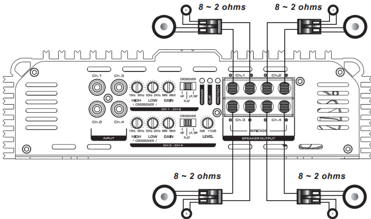
3-4D. WDX PRO 4 CHANNEL AMPLIFIERS' SPEAKER CONNECTION DIAGRAM 2.
