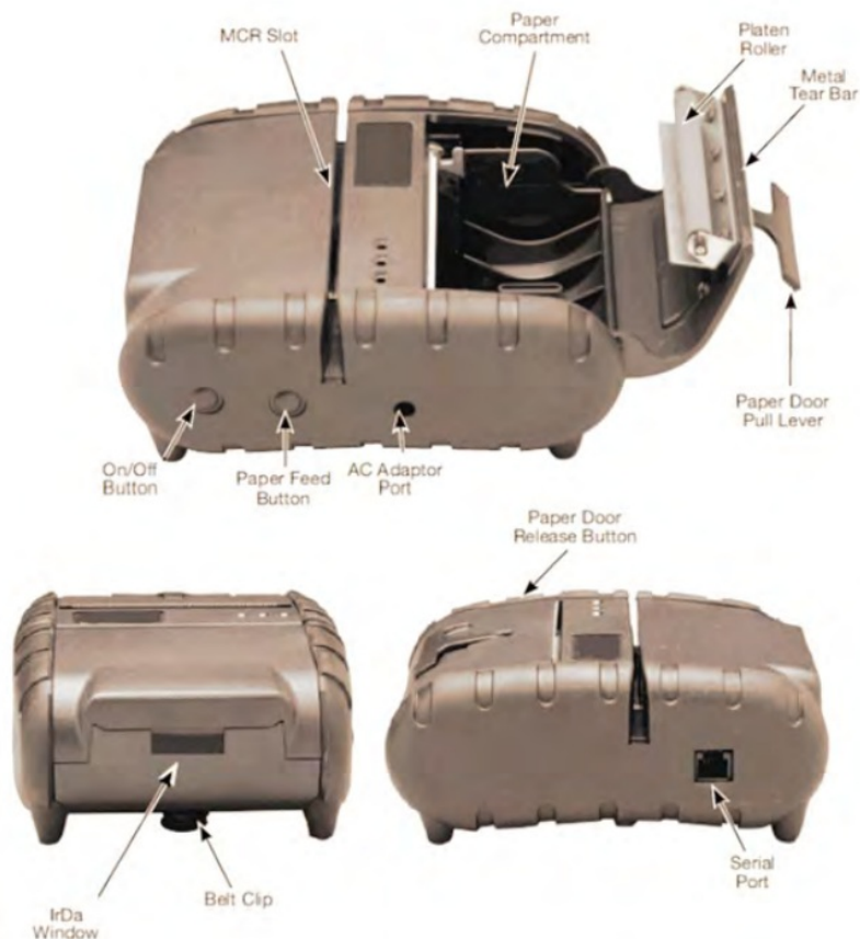
FIGURE 1: PRINTER OVERVIEW
