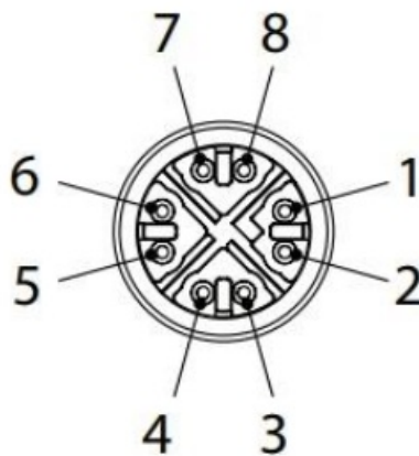
Matrix 220 Ethernet
