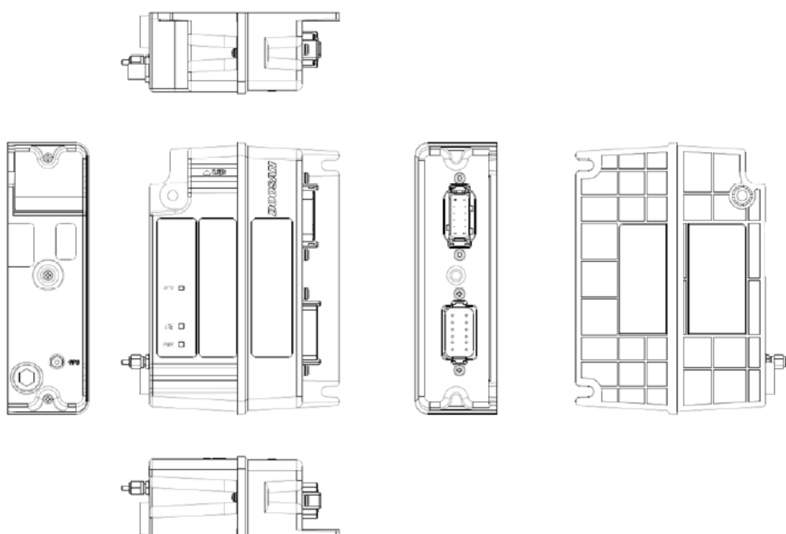
Fig. 3.1 Overall Shape Of TMS3.0 Type-A
