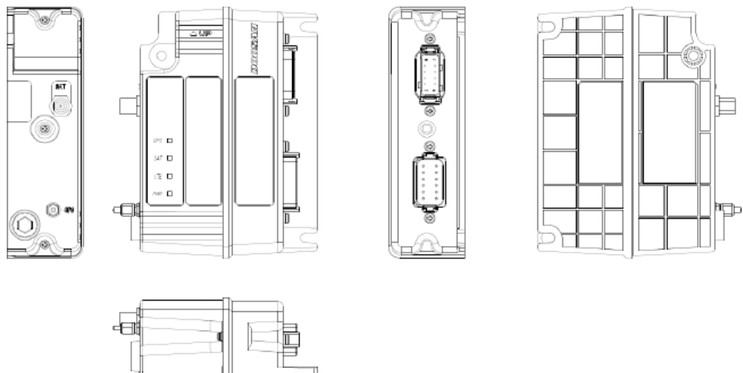
Fig. 3.2 Overall Shape Of TMS3.0 Type-B
