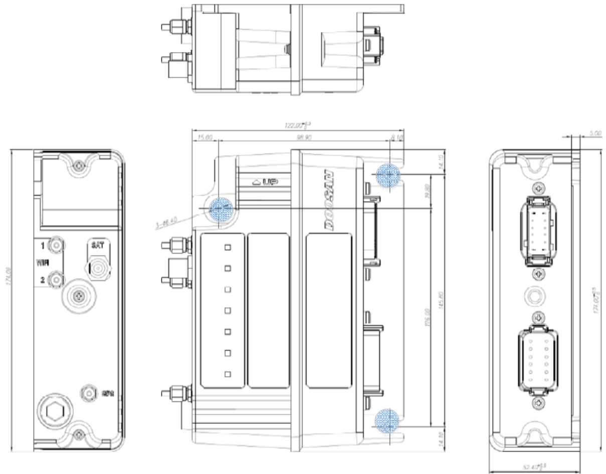
Fig. 4.1 Installation Block Diagram Of TMS3.0
